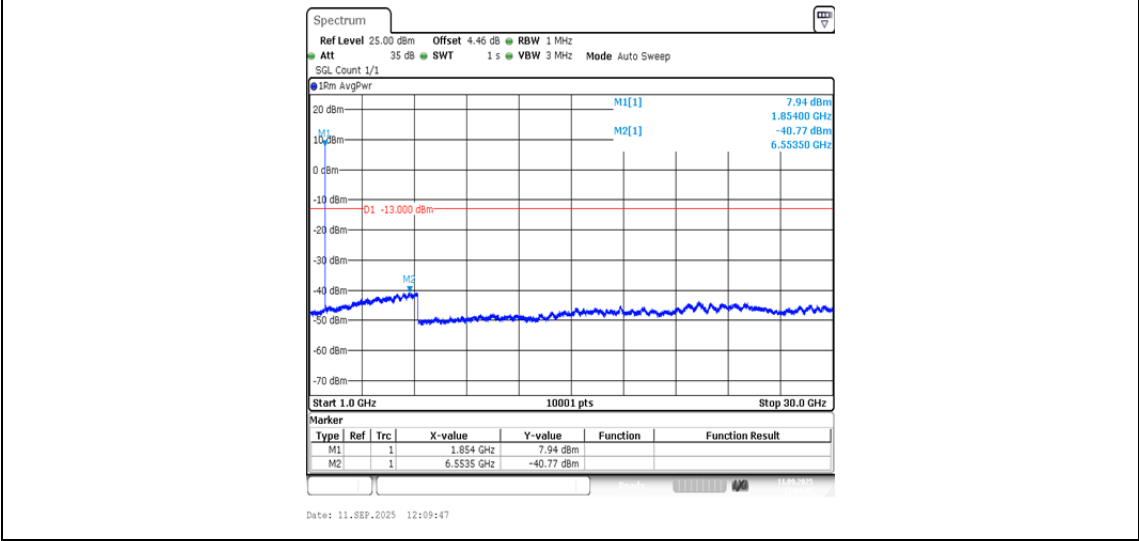
Band2-9262-2-1000~30000MHz-PASS
