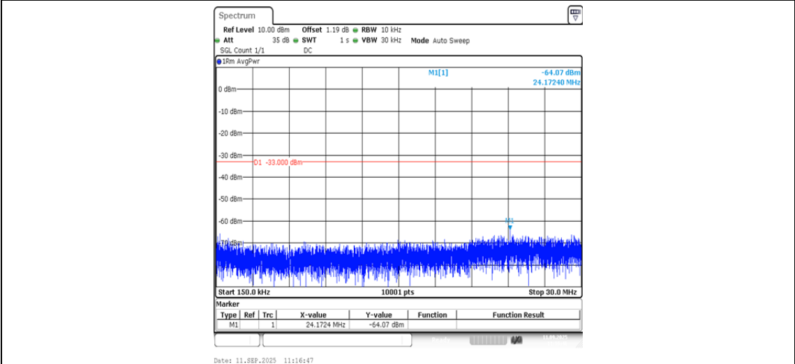
Band2-9400-2-0.15~30MHz-PASS
