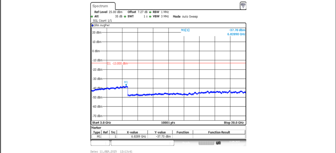
Band2-9262-3-3000~20000MHz-PASS
