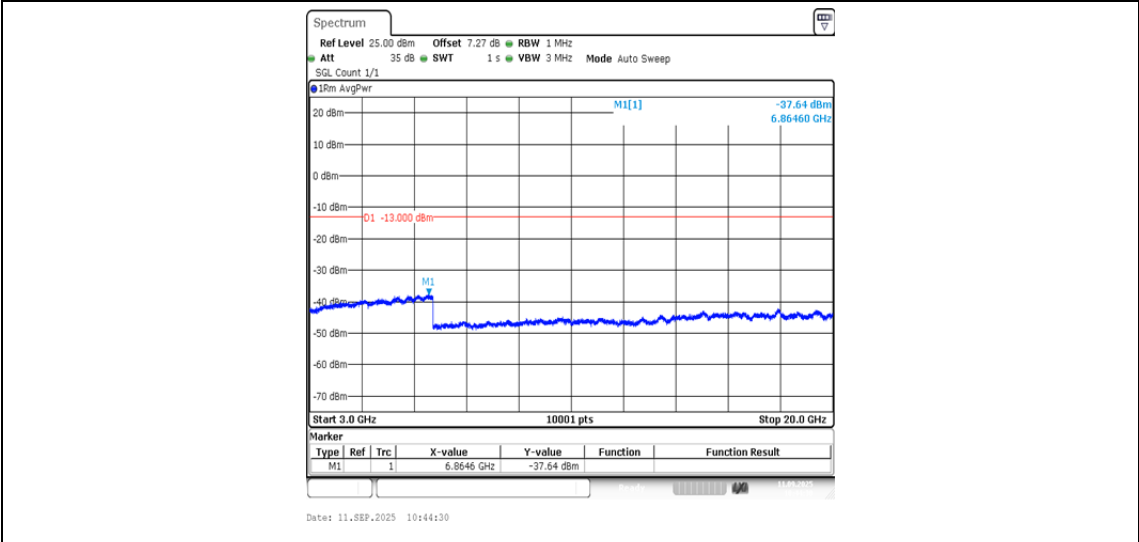
Band2-9262-3000~20000MHz-PASS
