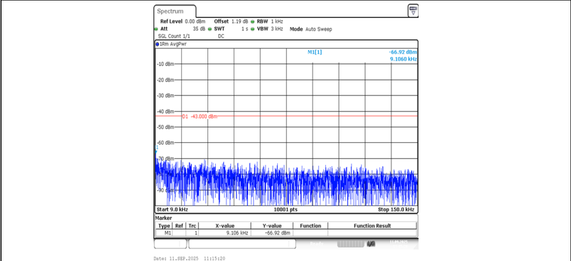
Band2-9262-2-0.009~0.15MHz-PASS
