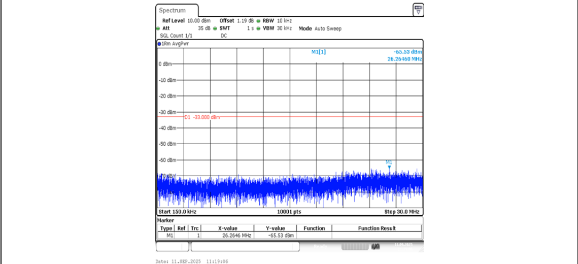
Band2-9262-3-0.15~30MHz-PASS
