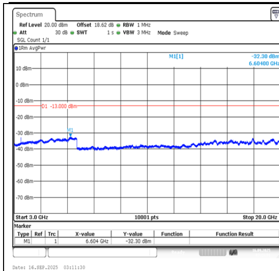
Band4-15MHz-QPSK-20025-1RB#0-3000~20000 -PASS
