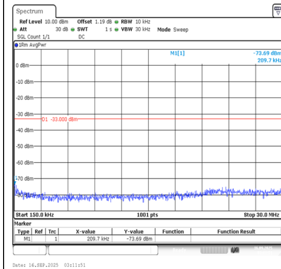
Band4-15MHz-16QAM-20025-1RB#0-0.15~30-PA SS
