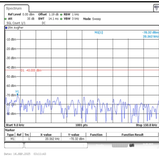
Band4-15MHz-16QAM-20025-1RB#0-0.009~0.15- PASS
