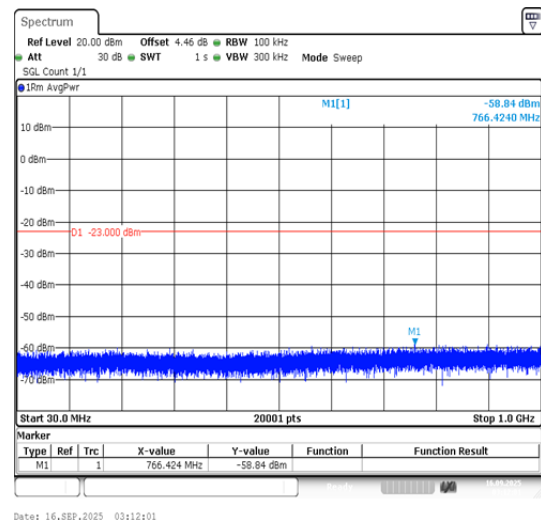
Band4-15MHz-16QAM-20025-1RB#0-30~1000-PA SS
