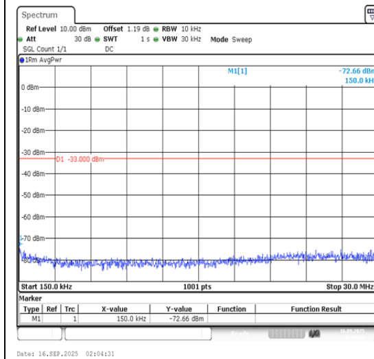
Band4-5MHz-16QAM-19975-1RB#0-0.15~30-PA
