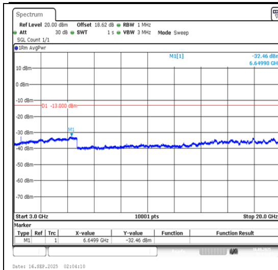
Band4-5MHz-QPSK-19975-1RB#0-3000~20000-PASS
