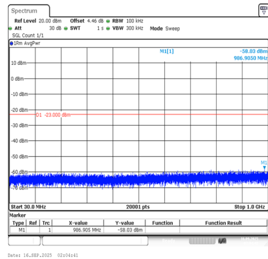
Band4-5MHz-16QAM-19975-1RB#0-30~1000-PASS
