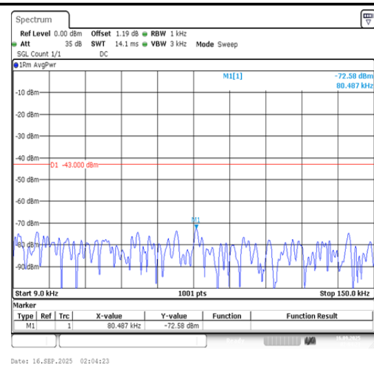
Band4-5MHz-16QAM-19975-1RB#0-0.009~0.15-PASS
