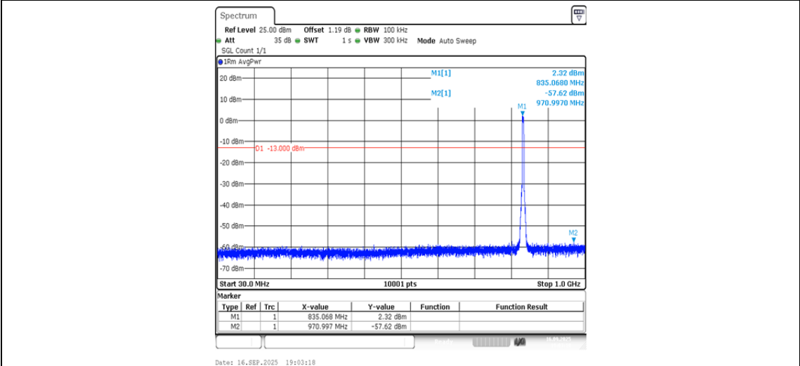
Band5-4182-2-30~1000MHz-PASS
