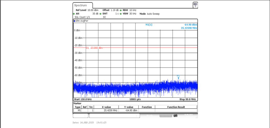
Band5-4132-2-0.15~30MHz-PASS
