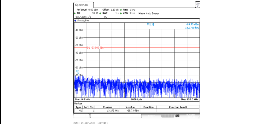
Band5-4132-3-0.009~0.15MHz-PASS
