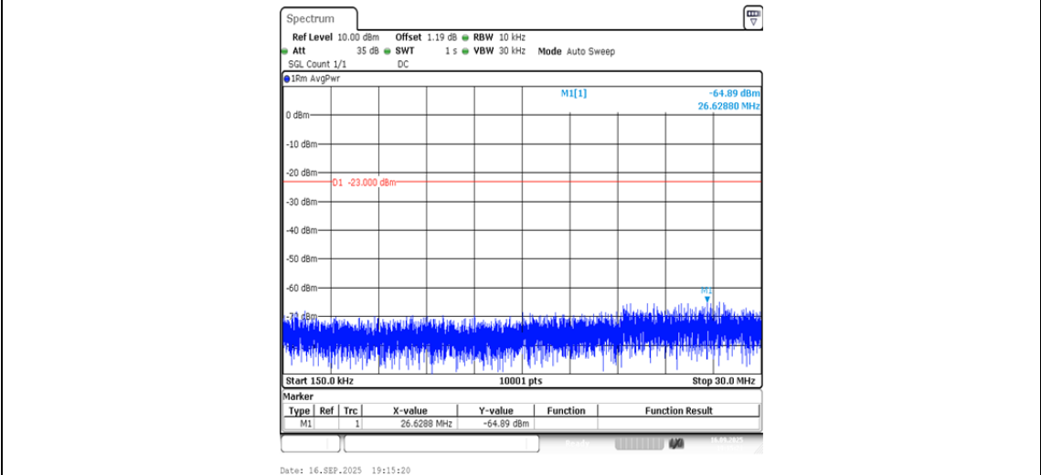
Band5-4132-5-0.15~30MHz-PASS
