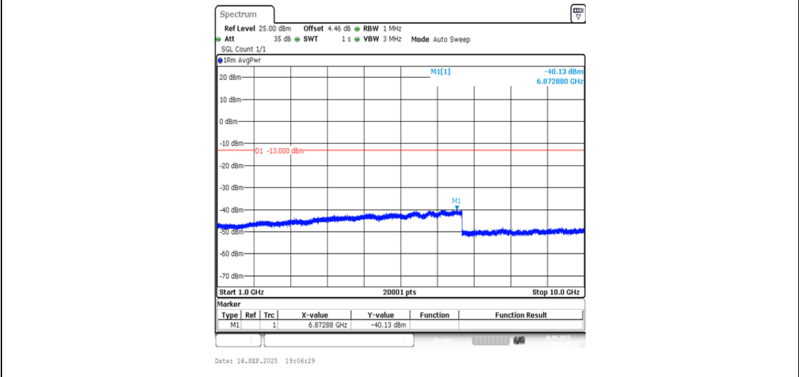
Band5-4132-3-1000~10000MHz-PASS
