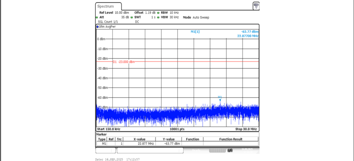
Band5-4182-0.15~30MHz-PASS
