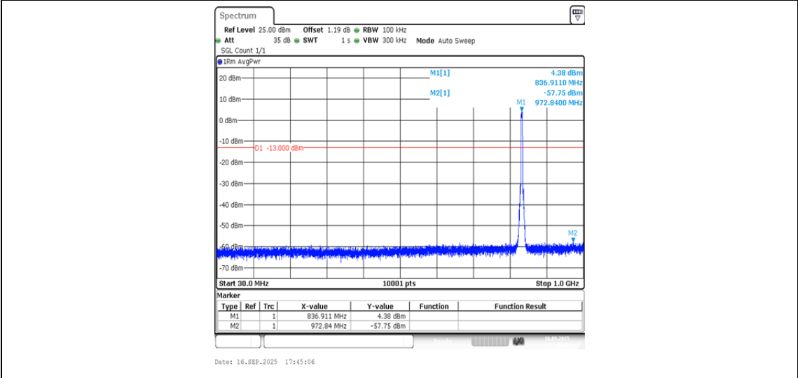
Band5-4182-3-30~1000MHz-PASS
