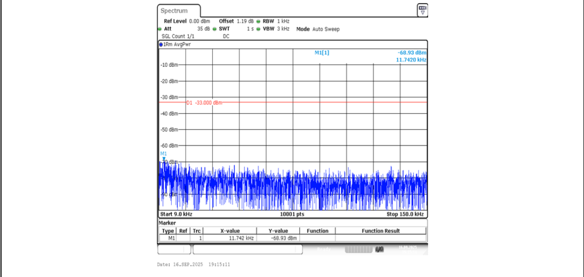
Band5-4132-5-0.009~0.15MHz-PASS
