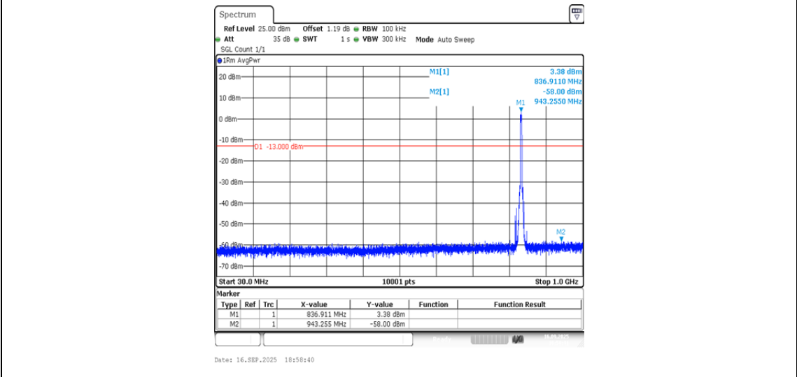
Band5-4182-1-30~1000MHz-PASS
