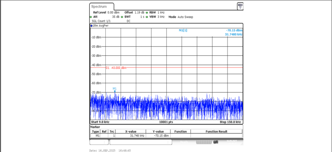
Band4-1513-1-0.009~0.15MHz-PASS
