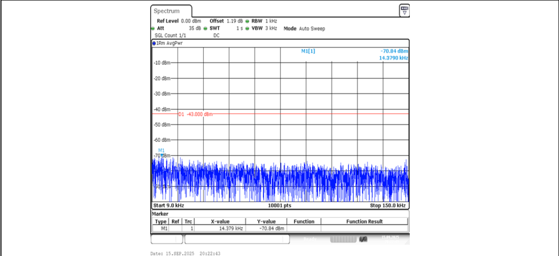
Band4-1413-1-0.009~0.15MHz-PASS
