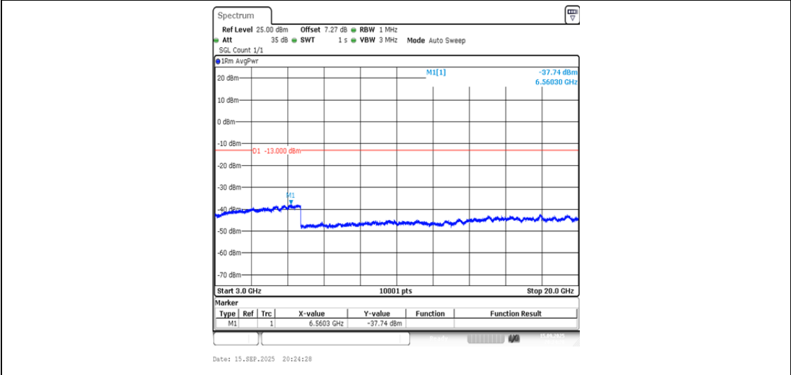
Band4-1513-1-3000~20000MHz-PASS
