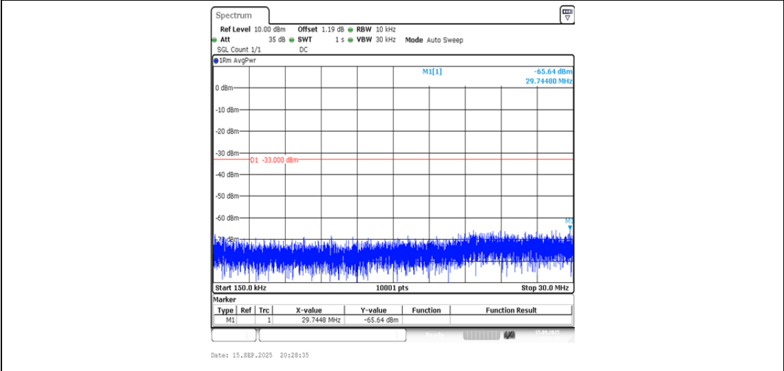
Band4-1312-3-0.15~30MHz-PASS
