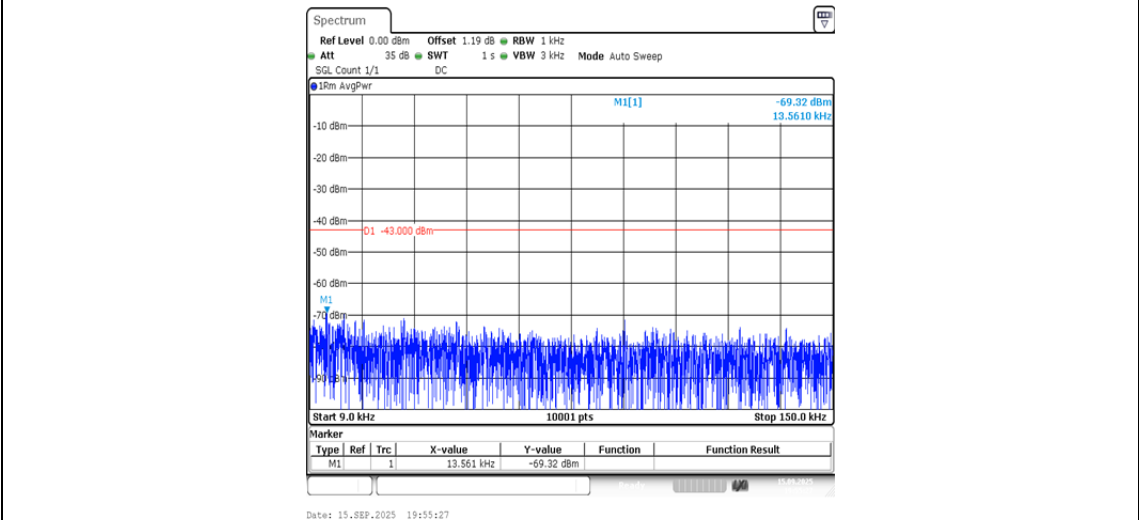
Band4-1413-0.009~0.15MHz-PASS
