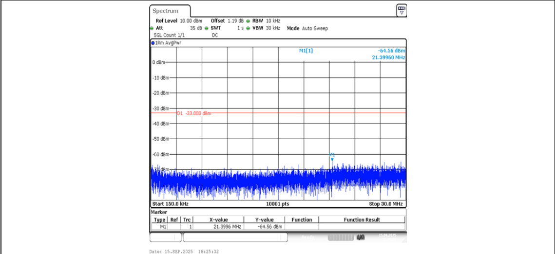
Band2-9538-4-0.15~30MHz-PASS
