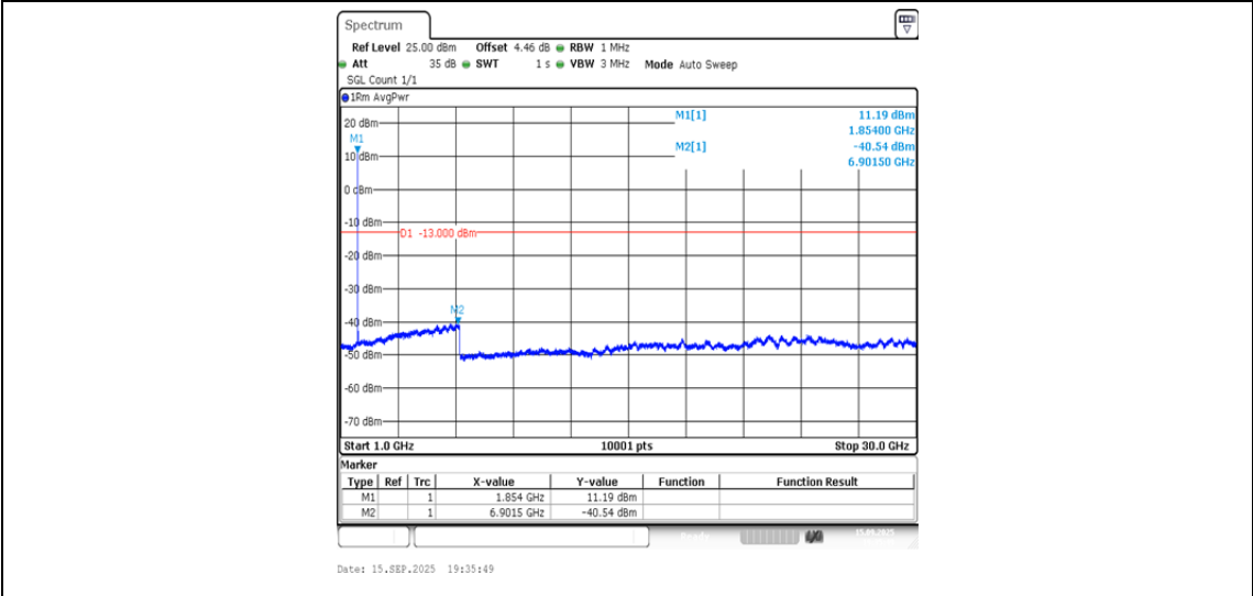
Band2-9262-3-1000~30000MHz-PASS
