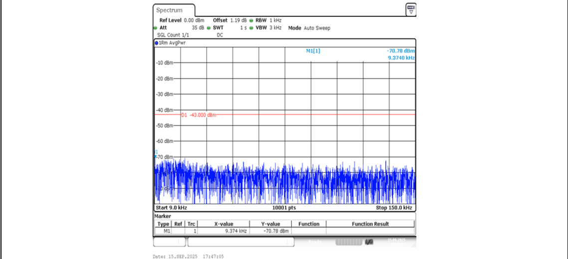
Band2-9400-0.009~0.15MHz-PASS
