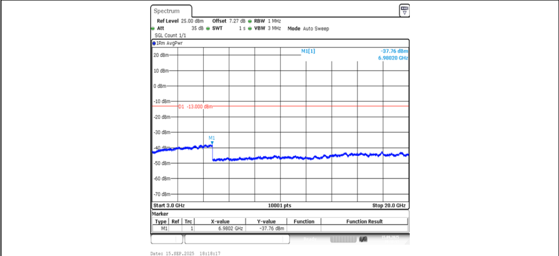
Band2-9400-2-3000~20000MHz-PASS
