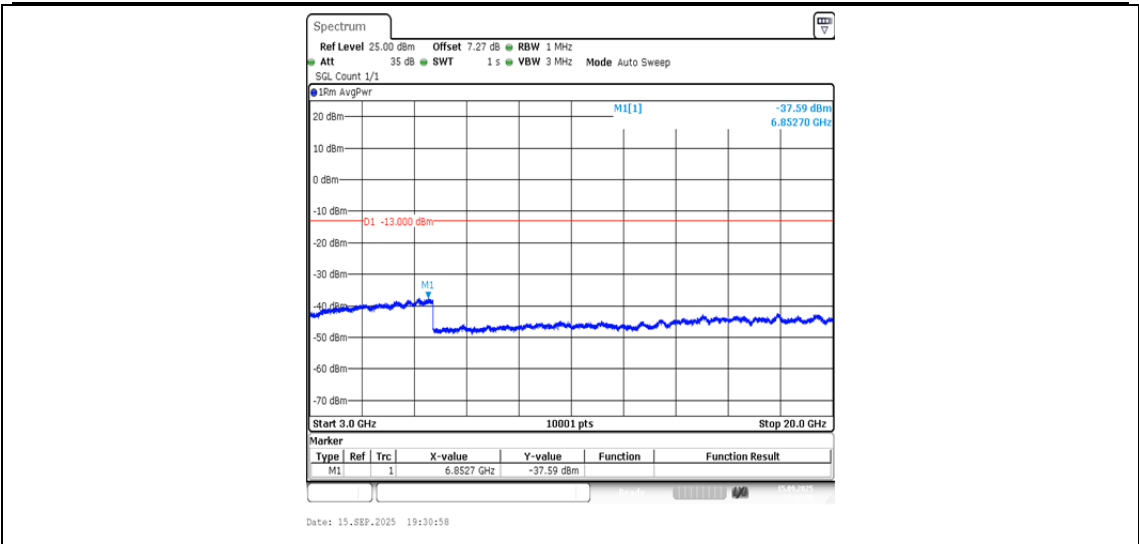
Band2-9262-2-3000~20000MHz-PASS
