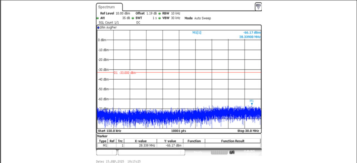
Band2-9538-1-0.15~30MHz-PASS
