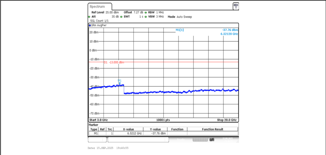
Band2-9262-4-3000~20000MHz-PASS
