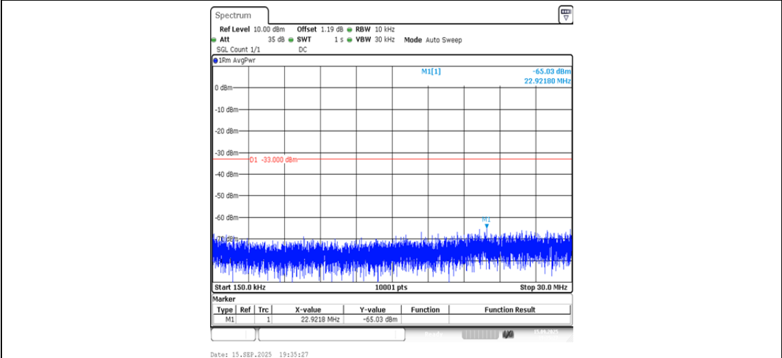
Band2-9262-3-0.15~30MHz-PASS
