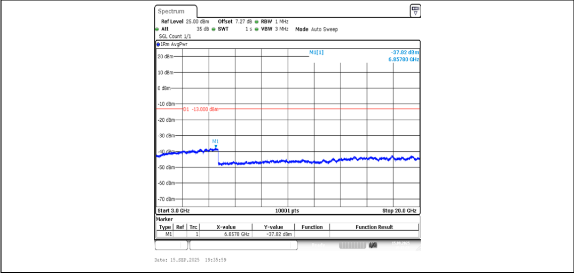
Band2-9262-3-3000~20000MHz-PASS
