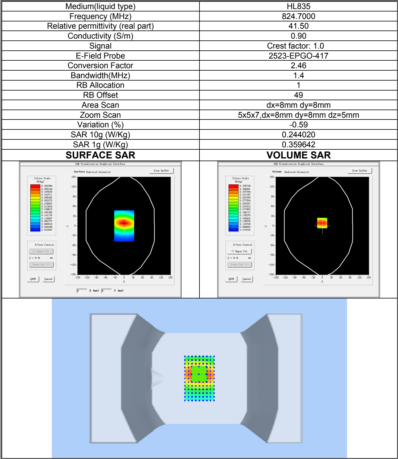
Plot 16: LTE BAND 5, Low channel (Body-worn/ Hotspot, Back Side) Product Description: Smart Phone Test Date: 2025-07-16
