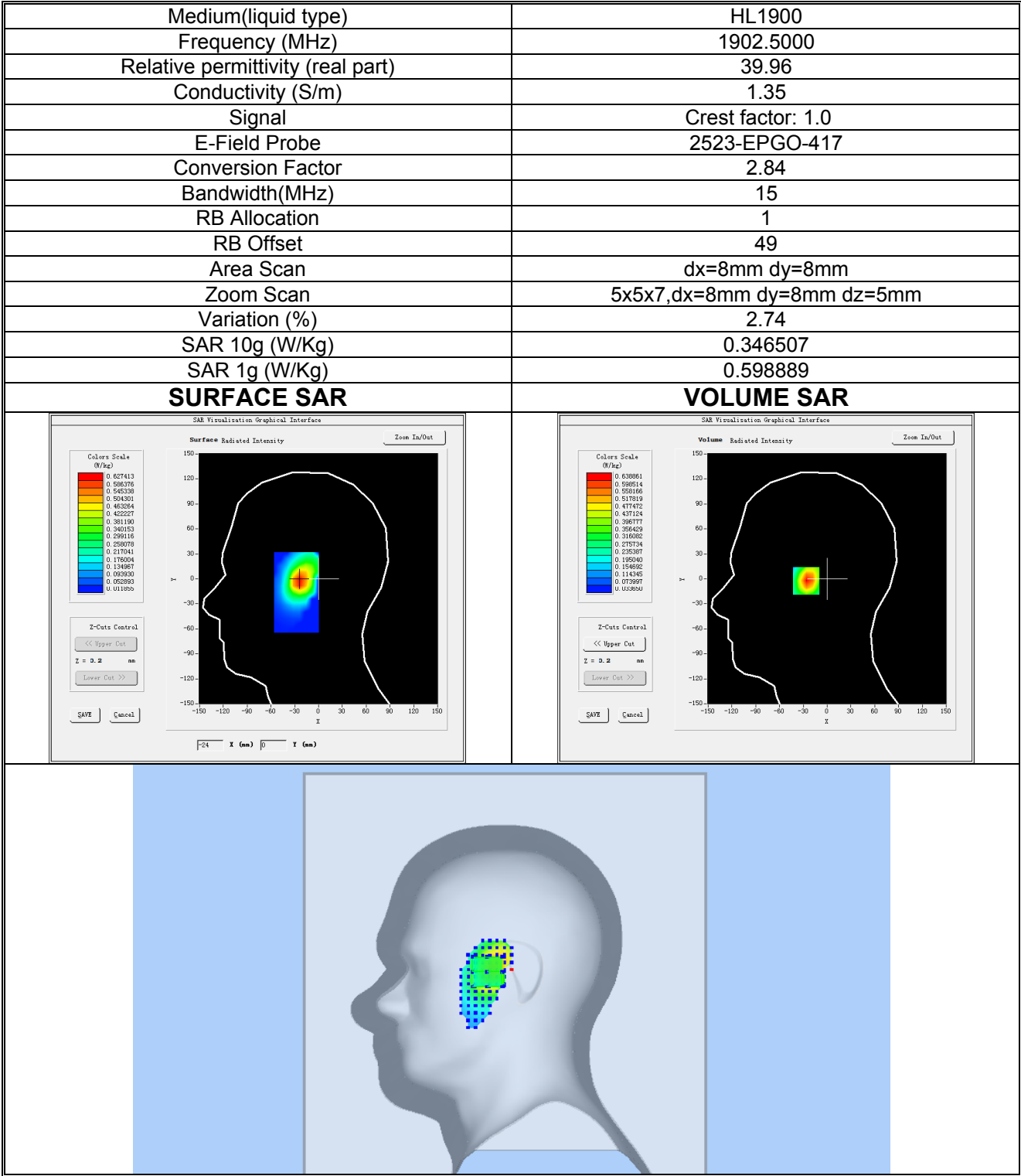
Plot 11:LTE BAND 2, High channel (Right Head Cheek) Product Description:Smart Phone Test Date: 2025-07-14
