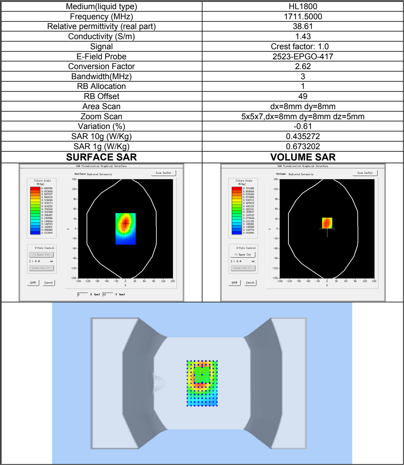
Plot 14: LTE BAND 4, Low channel (Body-worn/ Hotspot, Back Side) Product Description: Smart Phone Test Date: 2025-07-12
