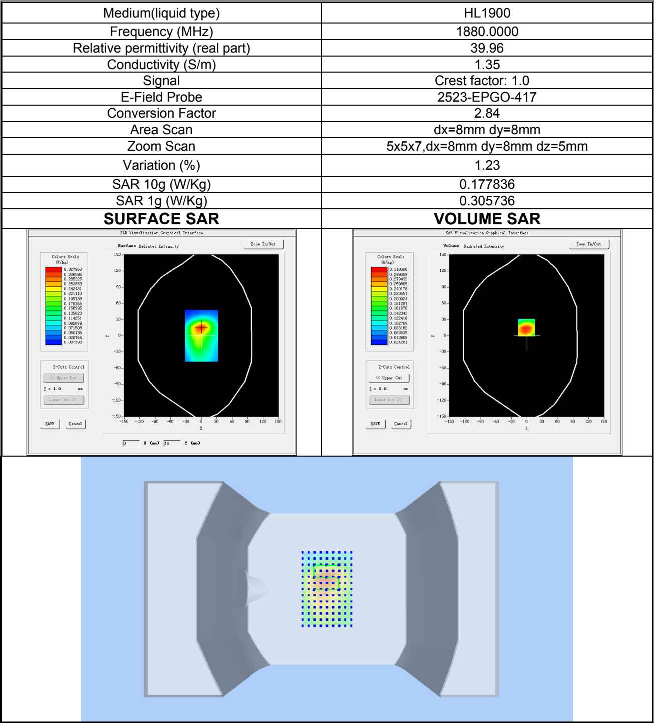
Plot 4: GSM 1900, Middle channel (Body-worn /Hotspot, Back Side) Product Description: Smart Phone Test Date: 2025-07-14
