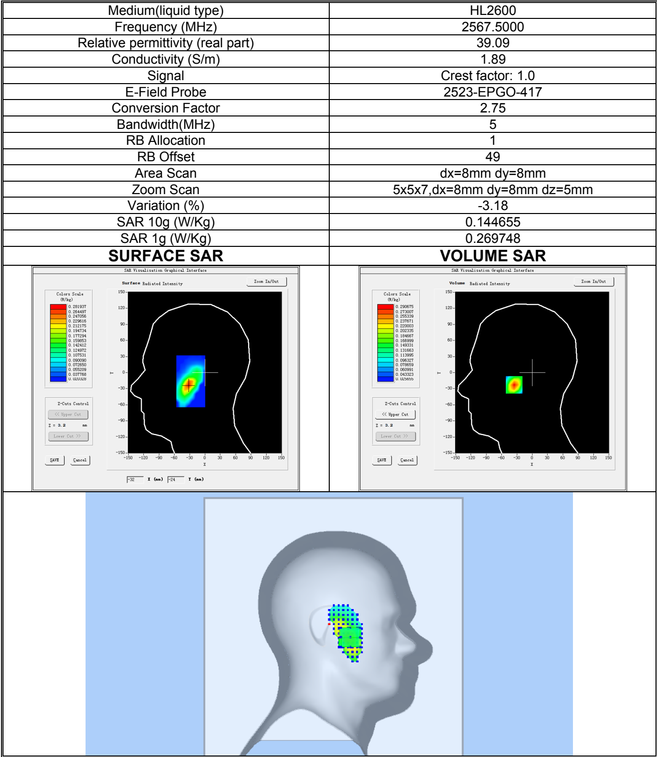
Plot 17:LTE BAND 7, High channel (Left Head Cheek) Product Description: Smart Phone Test Date: 2025-07-15
