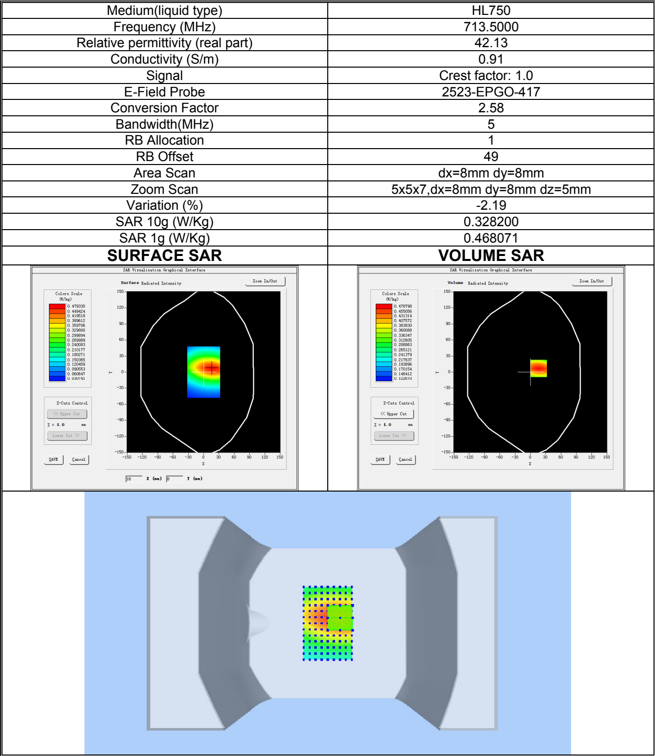
Plot 20: LTE BAND 12, High channel (Body-worn/ Hotspot, Back Side) Product Description: Smart Phone Test Date: 2025-07-16
