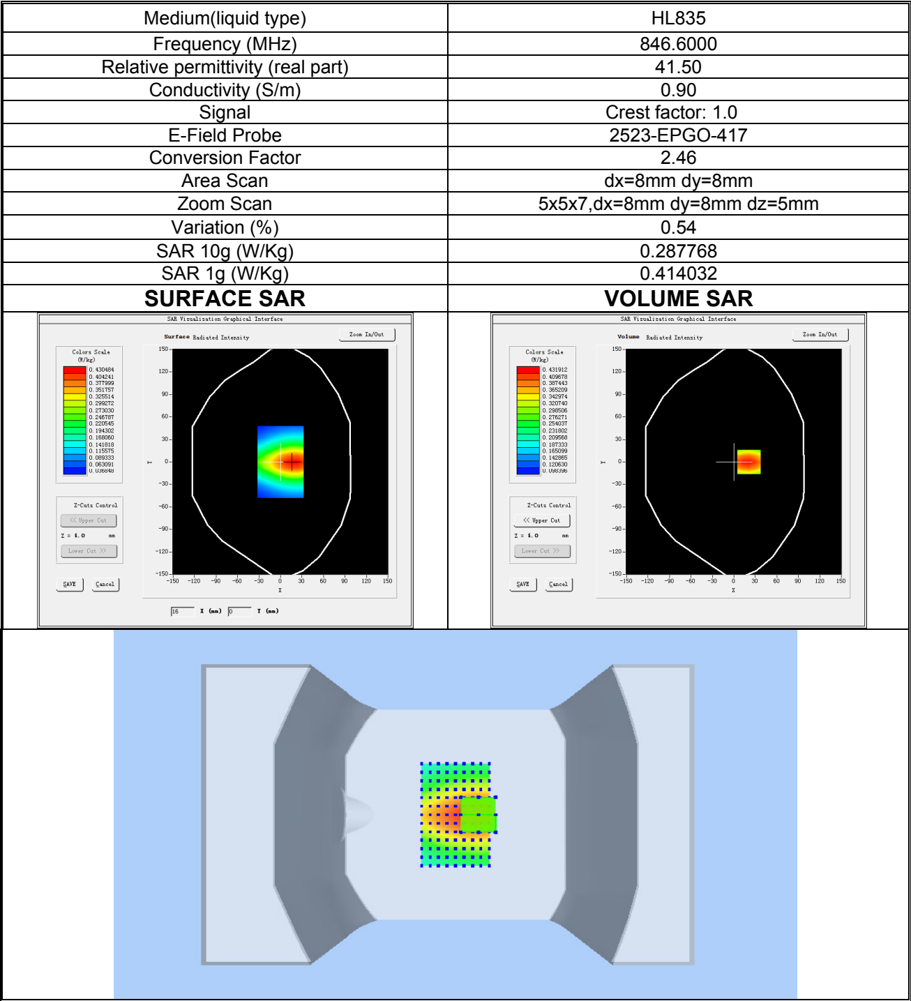
Plot 10: WCDMA BAND V, High channel (Body-worn/Hotspot, Left Edge) Product Description: Smart Phone Test Date: 2025-07-16
