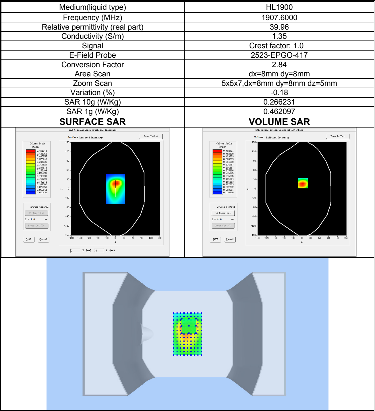
Plot 6: WCDMA BAND II, High channel (Body-worn /Hotspot, Back Side) Product Description: Smart Phone Test Date: 2025-07-14
