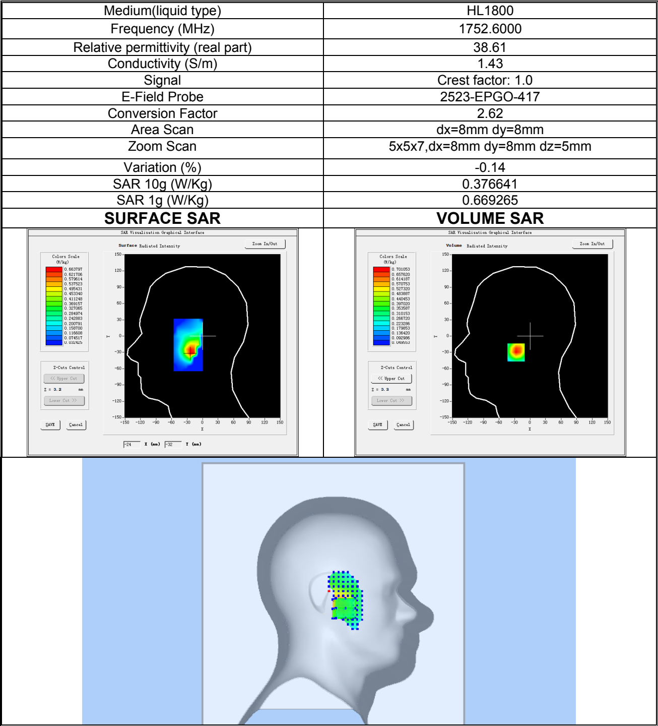
Plot 7: WCDMA BAND IV, High channel (Left Head Cheek) Product Description: Smart Phone Test Date: 2025-07-12
