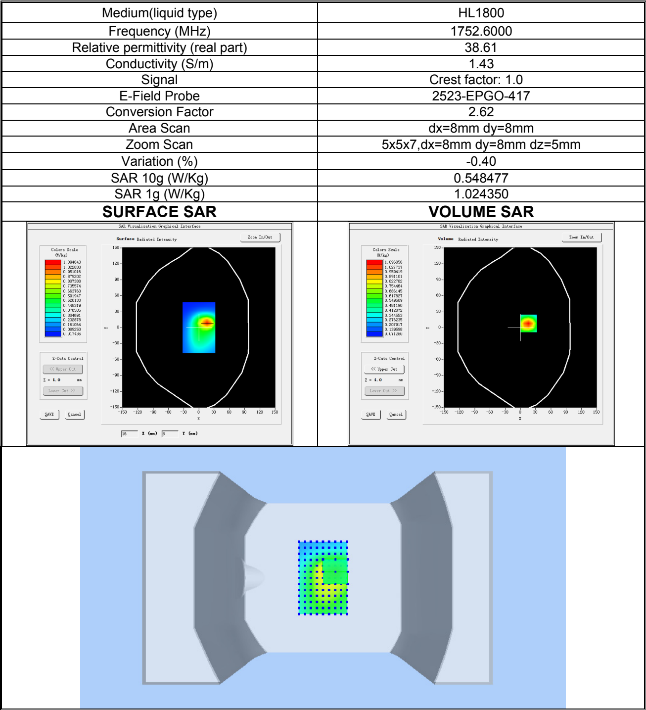
Plot 8: WCDMA BAND IV, High channel (Body-worn/Hotspot, Back Side) Product Description: Smart Phone Test Date: 2025-07-12
