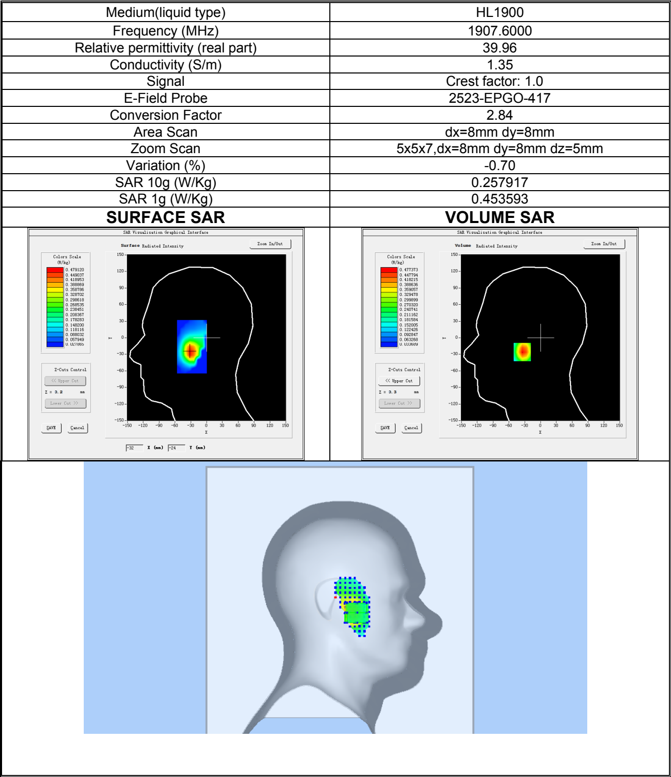
Plot 5: WCDMA BAND II, High channel (Left Head Cheek) Product Description: Smart Phone Test Date: 2025-07-14
