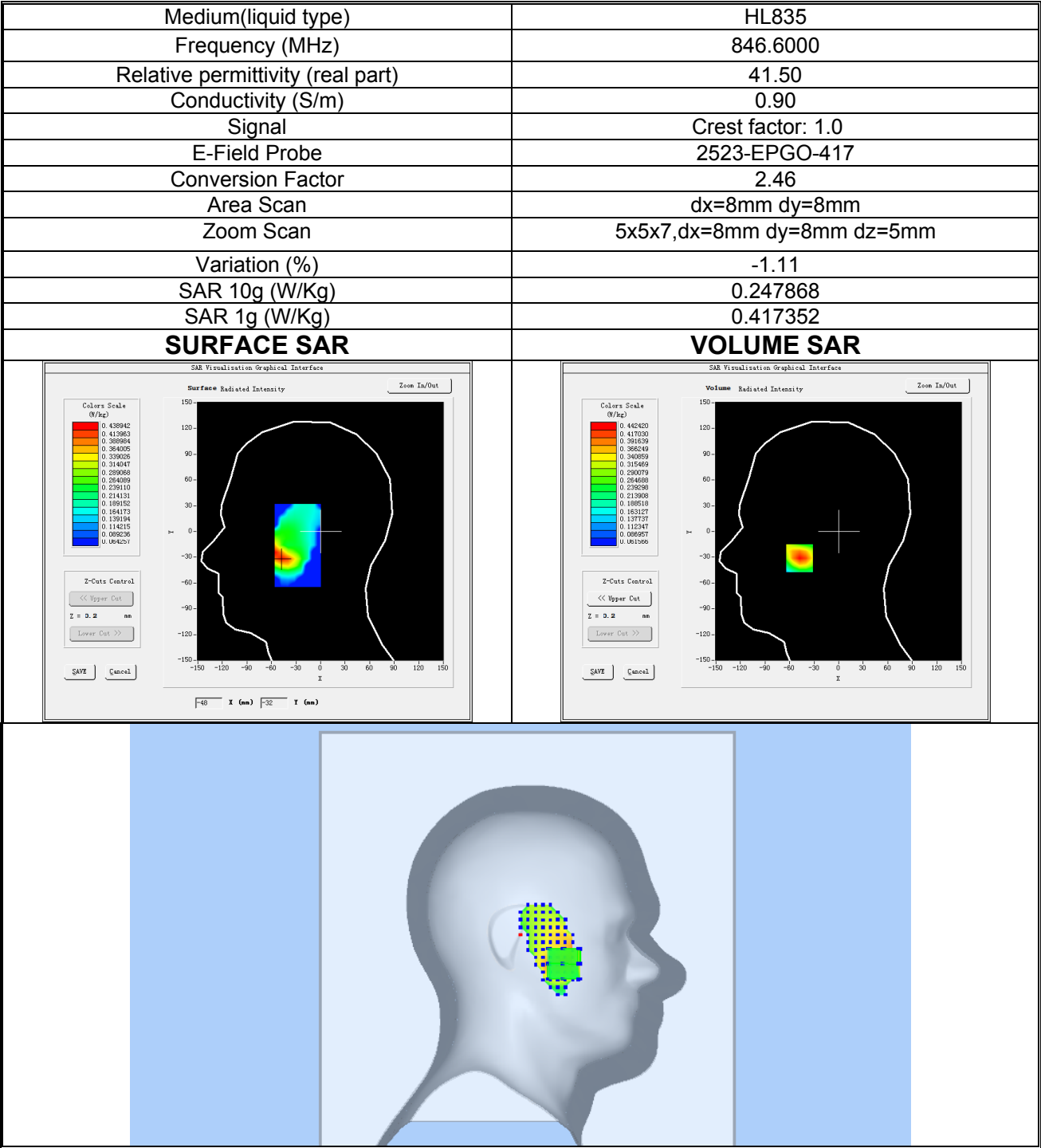
Plot 9: WCDMA BAND V, High channel (Left Head Cheek) Product Description: Smart Phone Test Date: 2025-07-16
