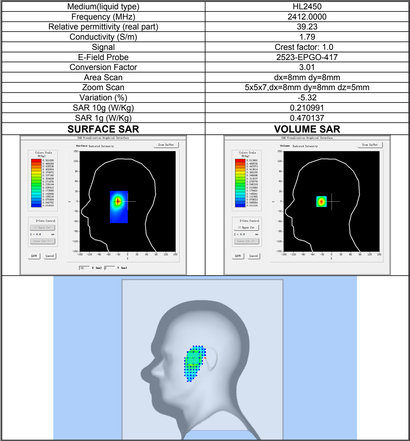
Plot 27:2.4G Wi-Fi, Low channel (Right Head Cheek) Product Description: Smart Phone Test Date: 2025-07-15
