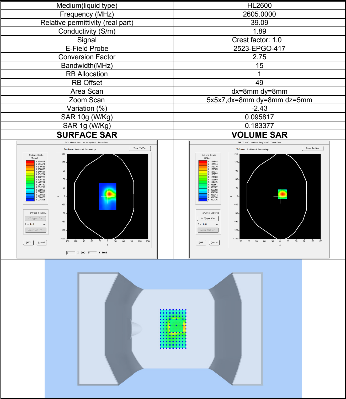
Plot 24: LTE BAND 41, Middle channel (Body-worn/ Hotspot, Back Side) Product Description: Smart Phone Test Date: 2025-07-15
