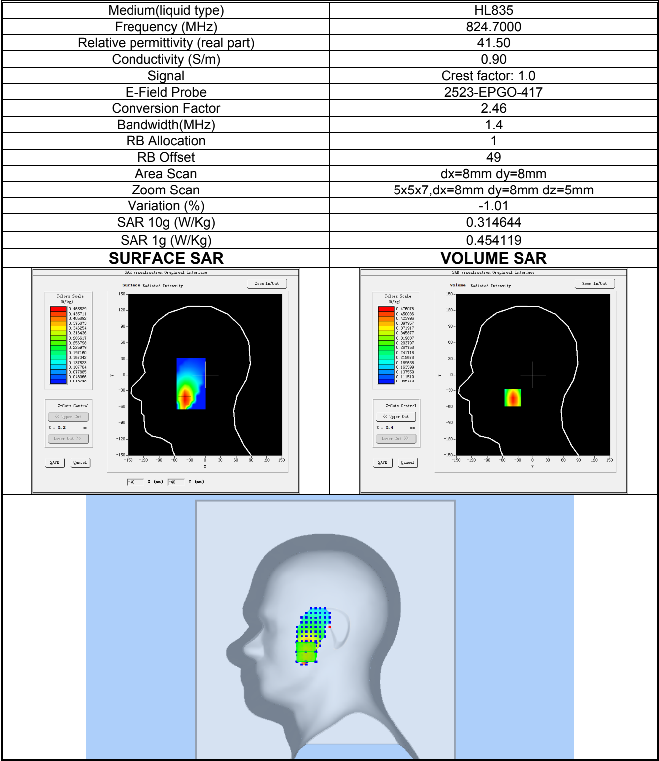
Plot 15:LTE BAND 5, Low channel (Right Head Cheek) Product Description: Smart Phone Test Date: 2025-07-16
