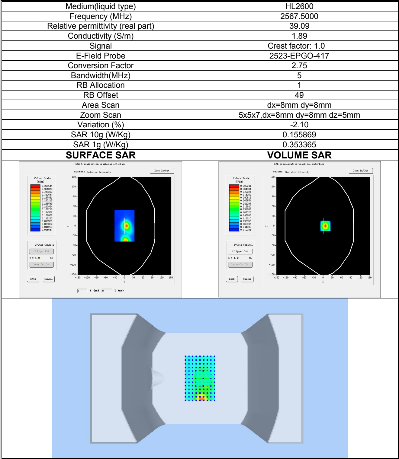
Plot 18: LTE BAND 7, High channel (Body-worn/ Hotspot, Bottom Edge) Product Description: Smart Phone Test Date: 2025-07-15
