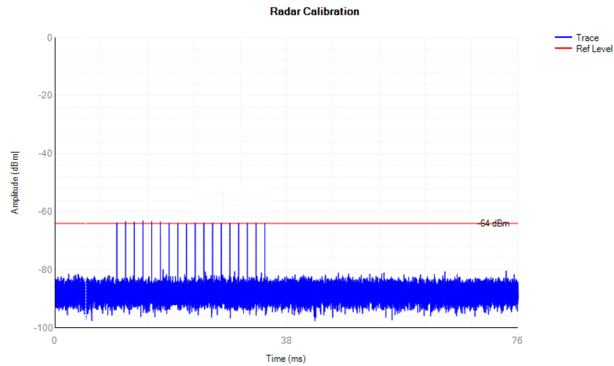
Radar Signal 5530
