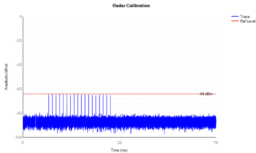
Radar Signal 5290
