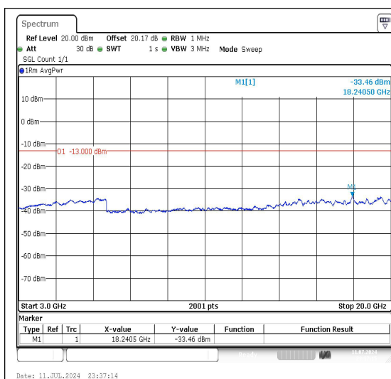
Band66_5MHz_QPSK_131997_1RB#0_3000~20000
