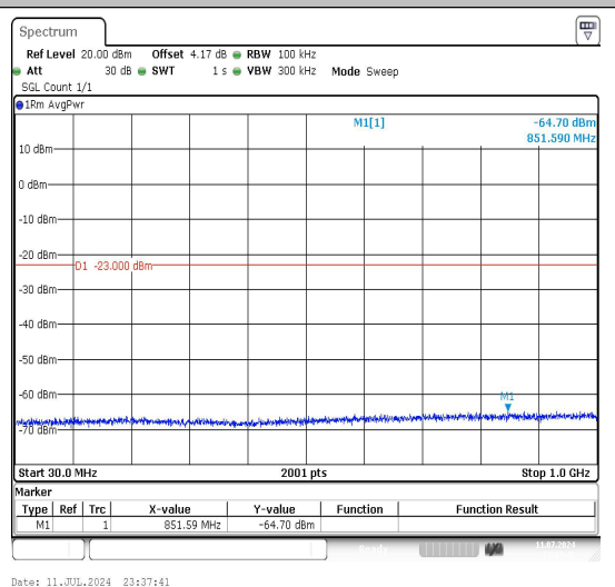
Band66_5MHz_16QAM_131997_1RB#0_30~1000
