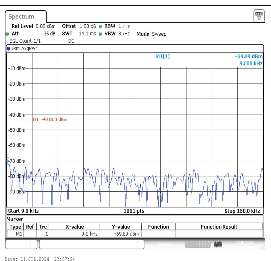
Band66_5MHz_16QAM_131997_1RB#0_0.009~0.15
