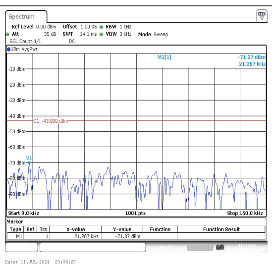
Band66_3MHz_16QAM_131987_1RB#0_0.009~0.15
