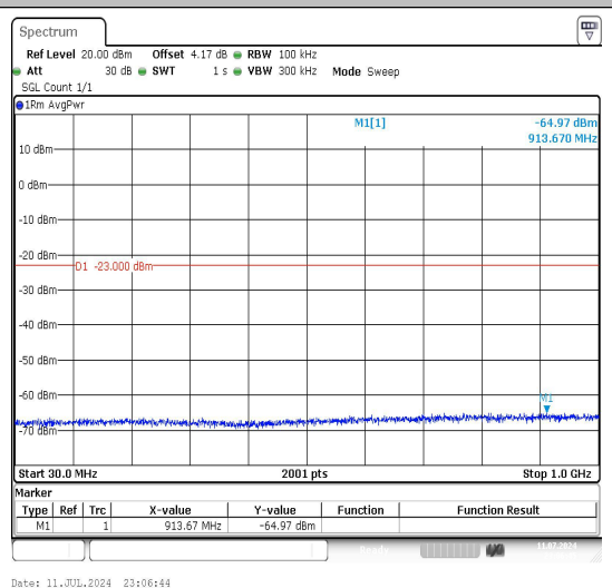
Band66_3MHz_16QAM_131987_1RB#0_30~1000
