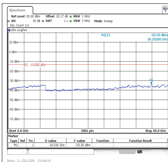
Band66_3MHz_QPSK_131987_1RB#0_3000~20000
