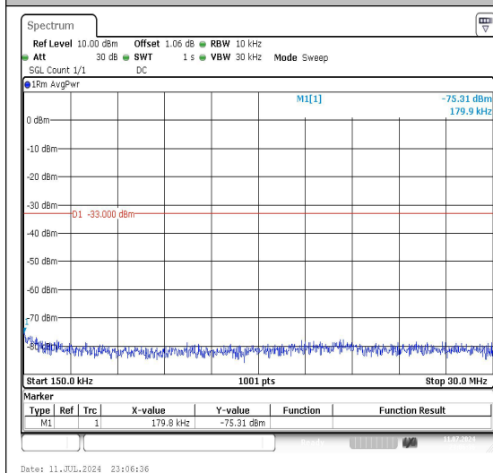
Band66_3MHz_16QAM_131987_1RB#0_0.15~3
