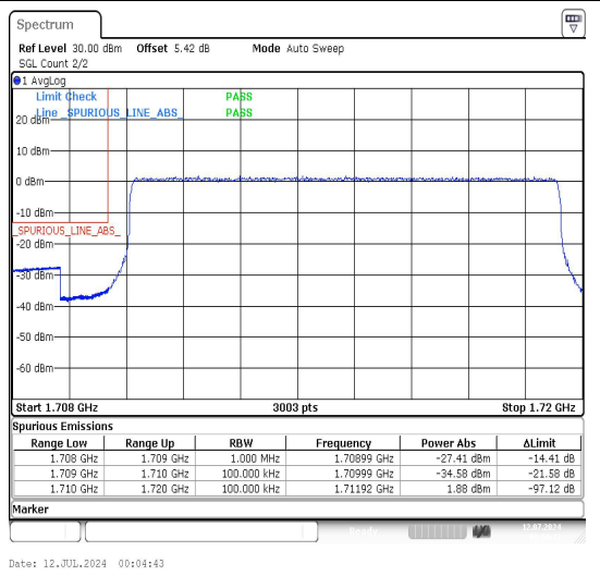
Band66_10MHz_16QAM_132022_50RB#0
