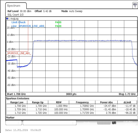
Band66_10MHz_QPSK_132022_50RB#0
