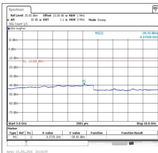
Band12_10MHz_QPSK_23060_1RB#0_3000~10000
