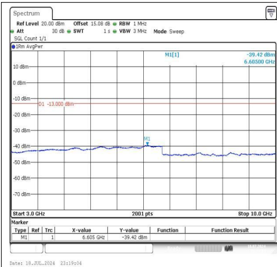
Band12_10MHz_QPSK_23130_1RB#0_3000~10000
