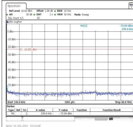
Band12_3MHz_16QAM_23165_1RB#0_0.15~30_0.15~30
