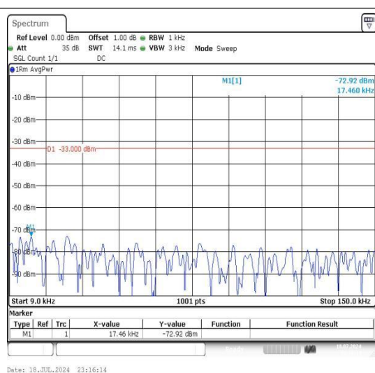
Band12_10MHz_16QAM_23060_1RB#0_0.009~0.15
