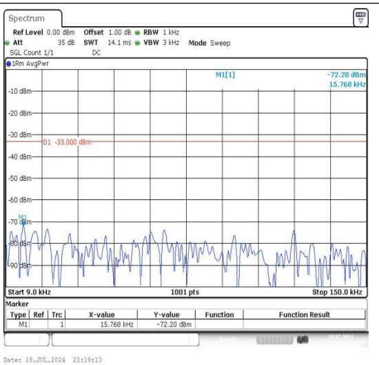
Band12_10MHz_16QAM_23130_1RB#0_0.009~0.15
