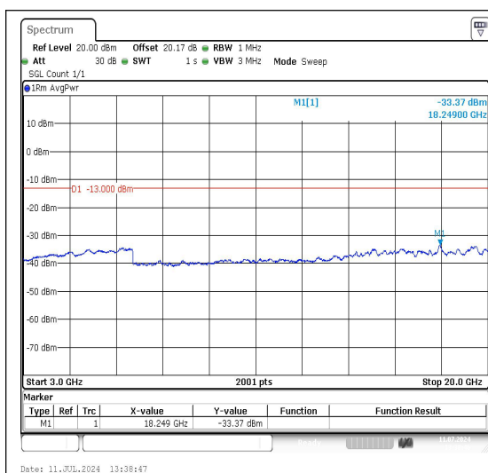
Band4_15MHz_QPSK_20325_1RB#0_3000~20000_3000~20000
