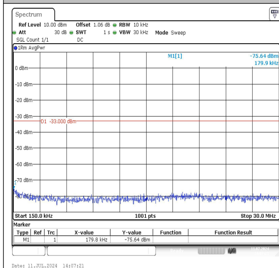
Band4_20MHz_16QAM_20050_1RB#0_0.15~30_0.15~30
