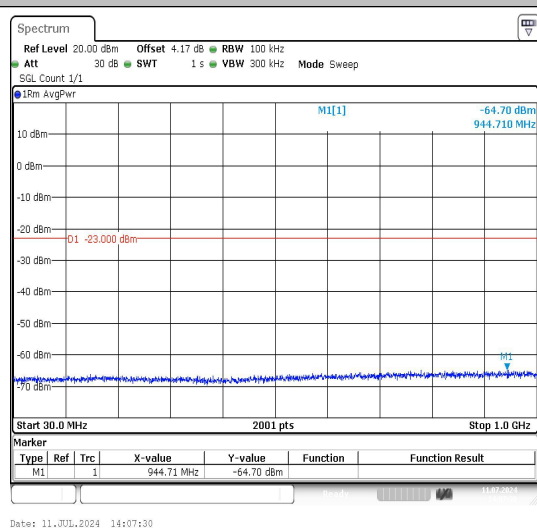
Band4_20MHz_16QAM_20050_1RB#0_30~1000_30~1000
