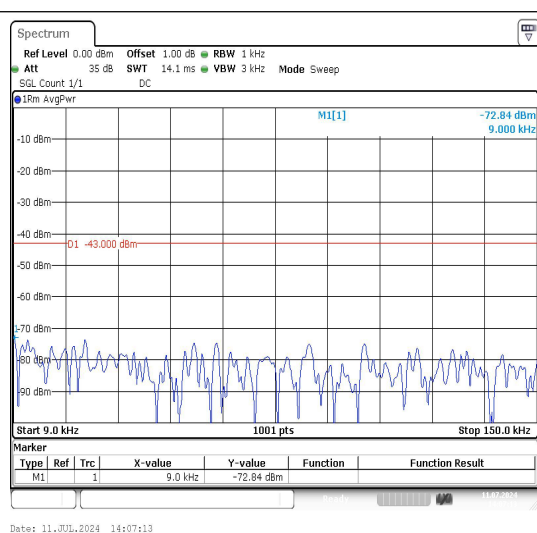
Band4_20MHz_16QAM_20050_1RB#0_0.009~0.15_0.009~0.15
