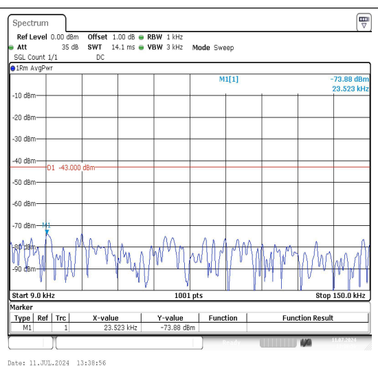
Band4_15MHz_16QAM_20325_1RB#0_0.009~0.15_0.009~0.15
