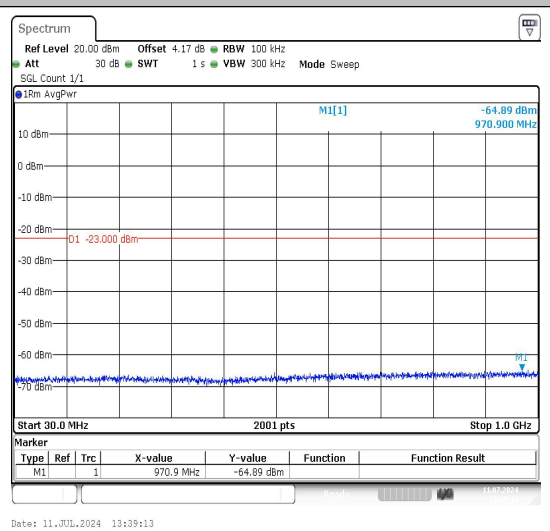
Band4_15MHz_16QAM_20325_1RB#0_30~1000_30~1000
