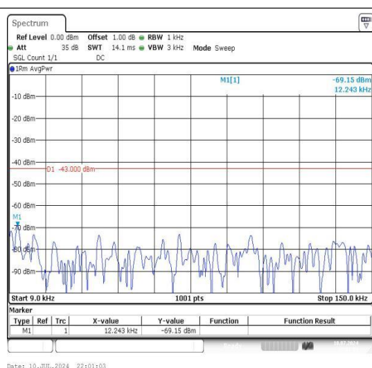
Band2_10MHz_16QAM_18650_1RB#0_0.009~0.15_0.009~0.15
