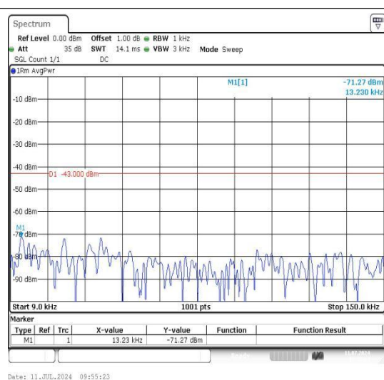
Band2_15MHz_16QAM_19125_1RB#0_0.009~0.15_0.009~0.15
