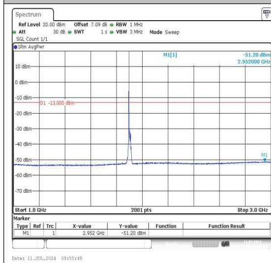
Band2_15MHz_16QAM_19125_1RB#0_0.15~30_0.15~30
