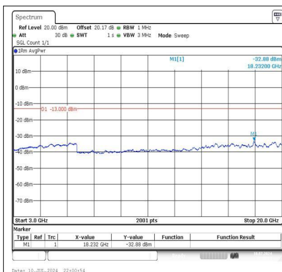
Band2_10MHz_QPSK_18650_1RB#0_3000~20000_3000~20000
