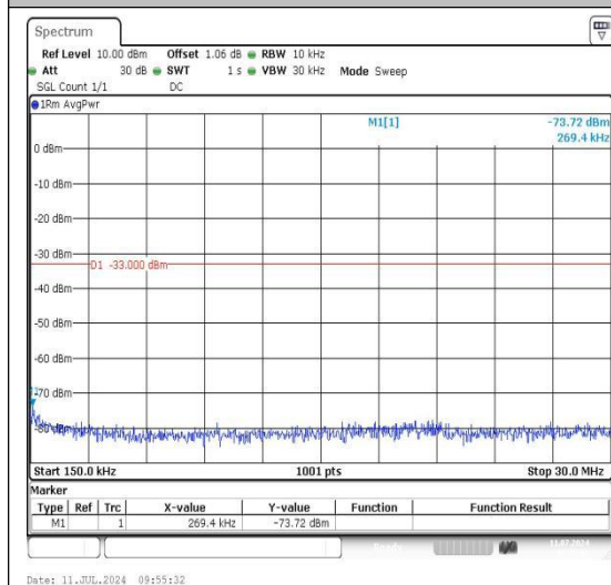
Band2_15MHz_16QAM_19125_1RB#0_0.15~30_0.15~30
