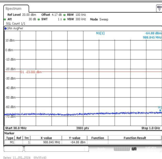
Band2_15MHz_16QAM_19125_1RB#0_30~1000_30~1000
