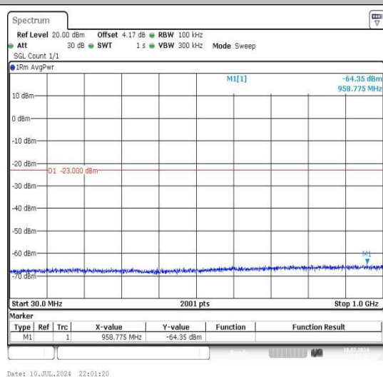
Band2_10MHz_16QAM_18650_1RB#0_30~1000_30~1000
