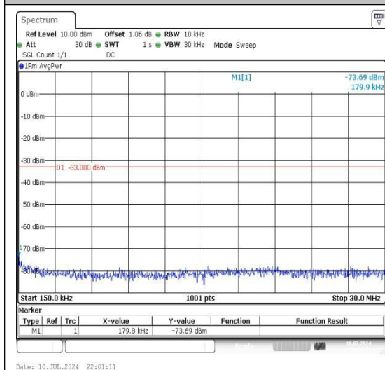
Band2_10MHz_16QAM_18650_1RB#0_0.15~30_0.15~30
