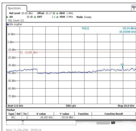
Band2_15MHz_QPSK_19125_1RB#0_3000~20000_3000~20000
