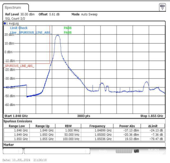
Band2_5MHz_16QAM_18625_1RB#0
