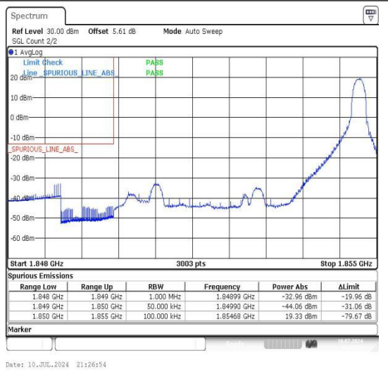
Band2_5MHz_16QAM_18625_1RB#24
