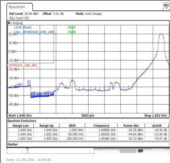
Band2_5MHz_QPSK_18625_1RB#24
