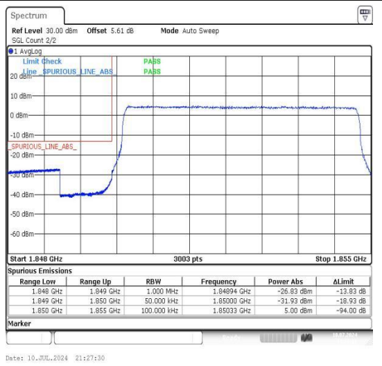
Band2_5MHz_16QAM_18625_25RB#0
