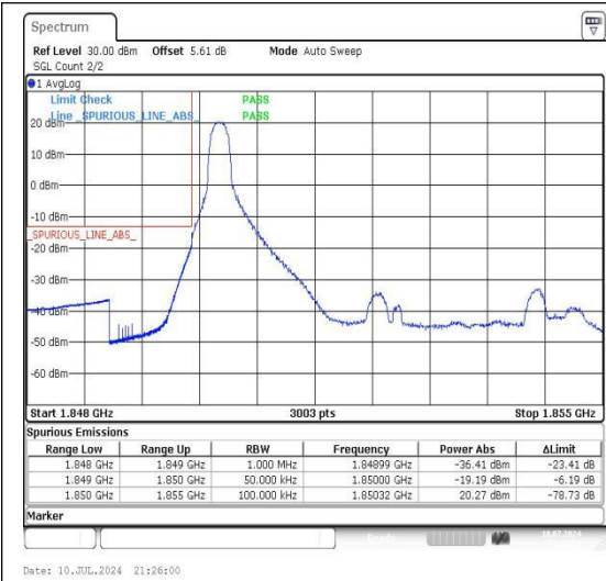
Band2_5MHz_QPSK_18625_1RB#0
