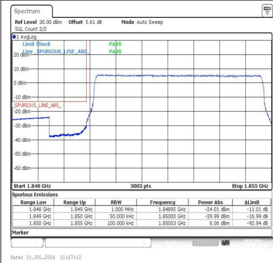
Band2_5MHz_QPSK_18625_25RB#0
