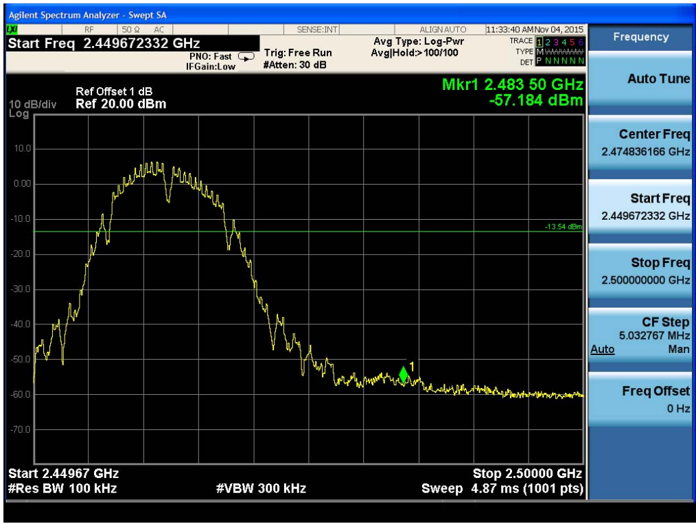
(Plot 4.5.2.1 B: Channel 11: 2462MHz @ 802.11 b )
