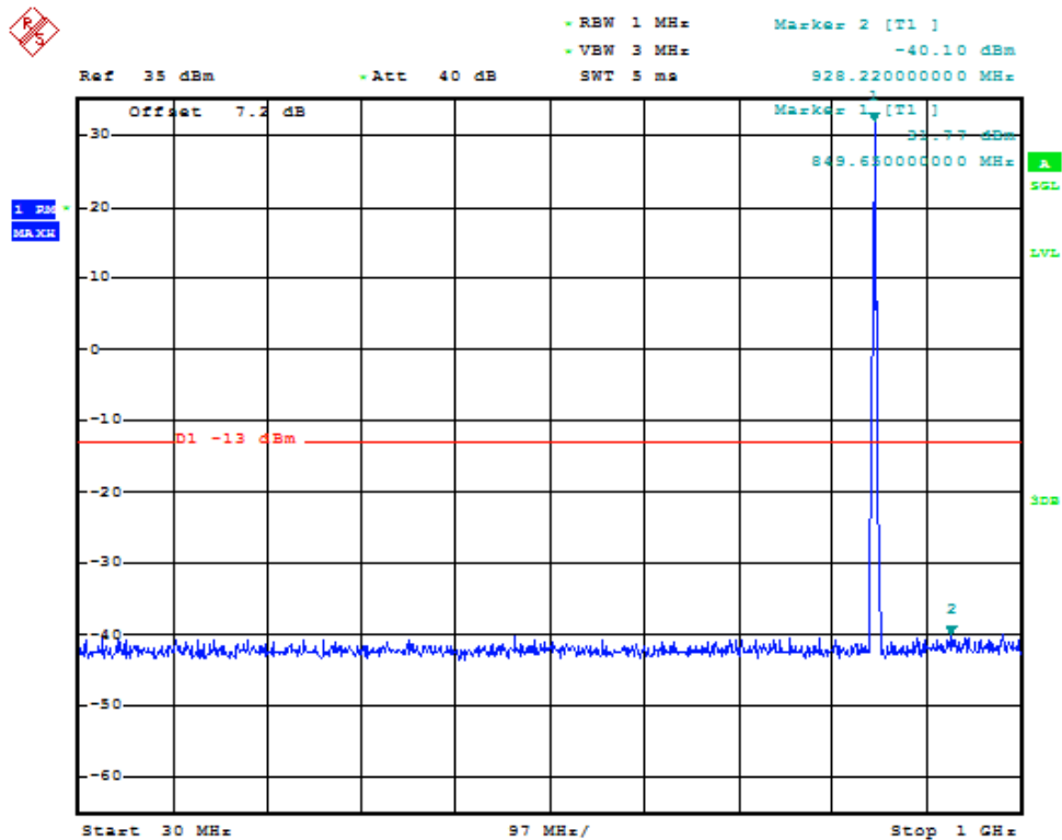
(Plot 4.5.1 C2: Channel 251: 848.80MHz @ Traffic @ GSM850)
