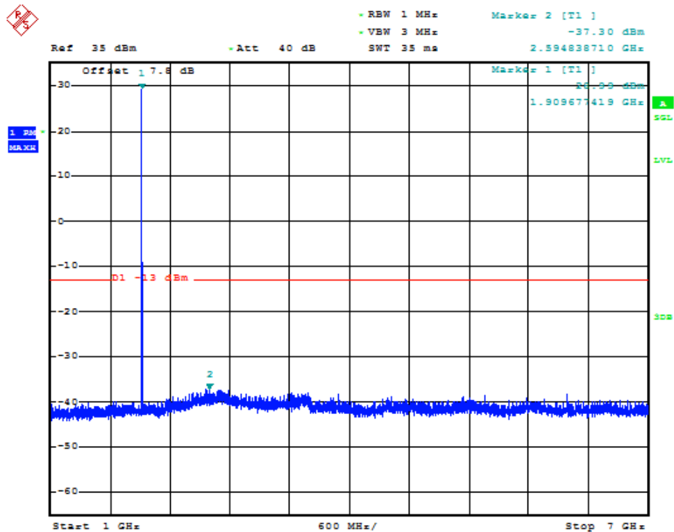
(Plot 4.5.2 C3: Channel 810: 1909.80MHz @ Traffic @ PCS1900)
