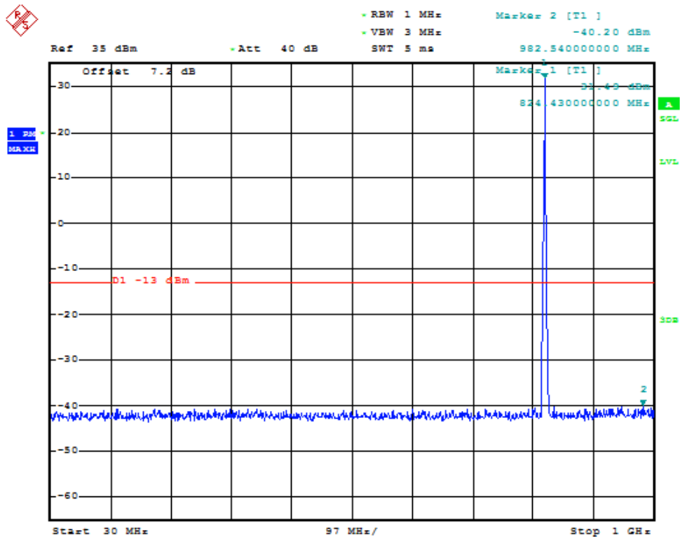
(Plot 4.5.1 A2: Channel 128: 824.20MHz @ Traffic @ GSM850)
