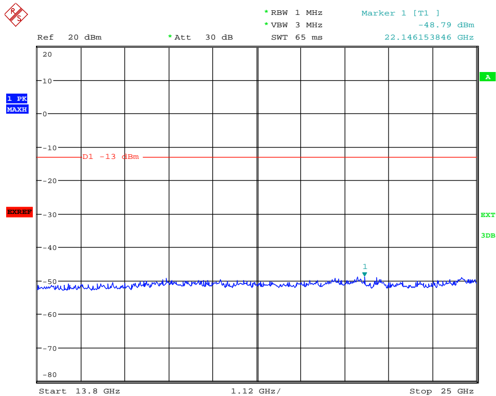
(Plot 4.5.1 C6: Channel 9538: 1907.6MHz @ Traffic WCDMA Band II)
