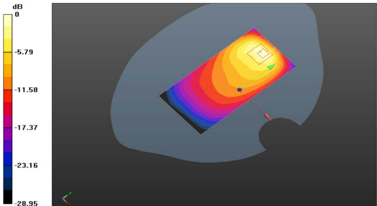
Plot 4: Body Rear Side (GSM1900 GPRS 4TS Hotspot Middle Channel)
