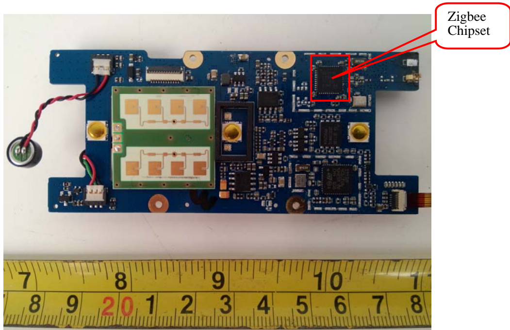
EUT – Main Board -2 Top shielding Cover off View
