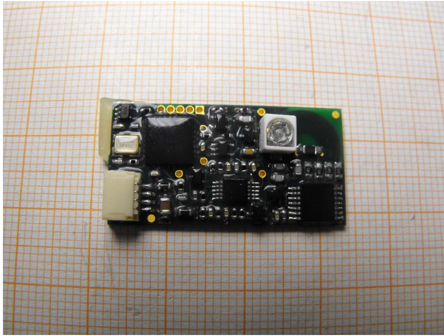
Photo 2: Module board rear side
