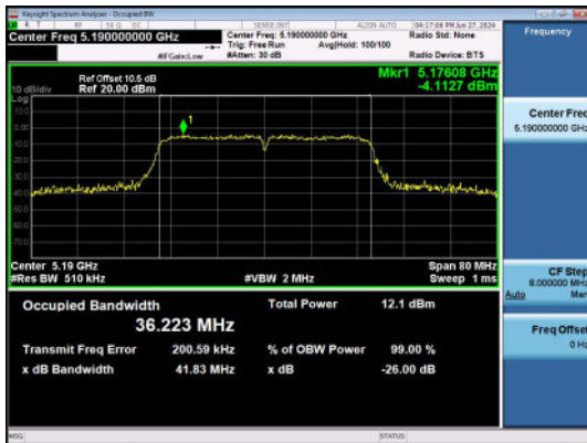
11N40SISO-Ant1-5190-99% OBW
