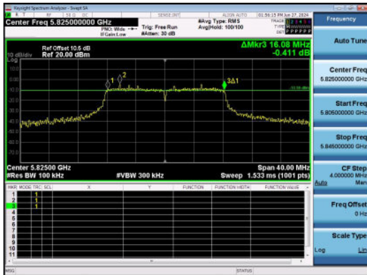
11A-Ant1-5825-PASS
