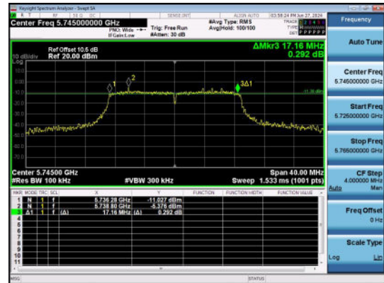
11N20SISO-Ant1-5745-PASS
