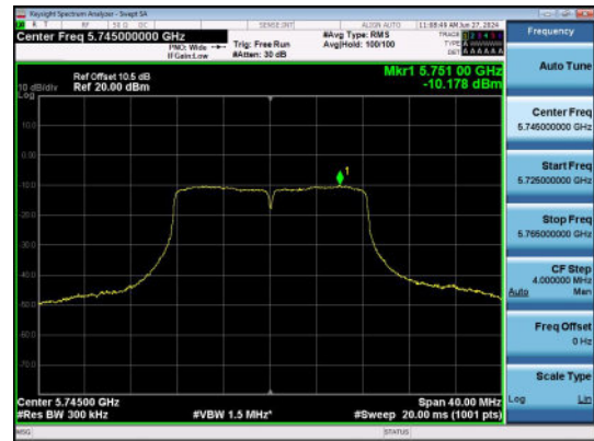
11A-Ant1-5745-PASS
