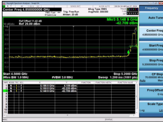
11A-Ant1-5180-PASS
