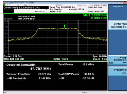
11A-Ant1-5220-99% OBW
