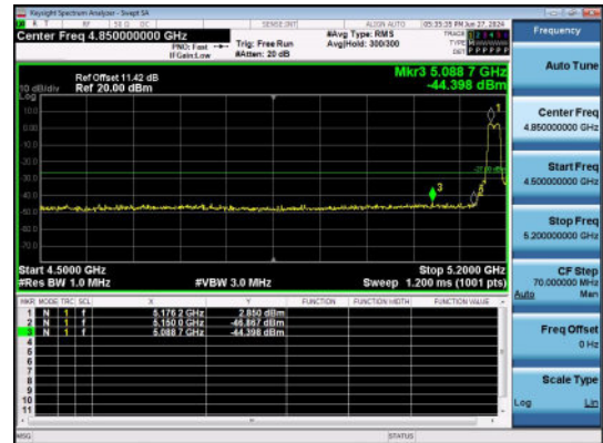
11AC20SISO-Ant1-5180-PASS
