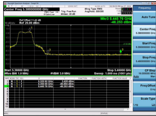
11N20SISO-Ant1-5320-PASS
