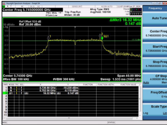
11A-Ant1-5745-PASS
