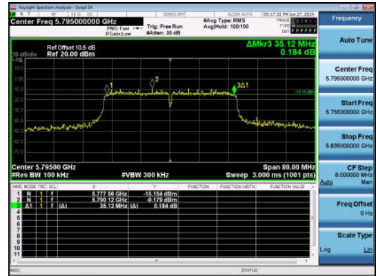
11N40SISO-Ant1-5795-PASS
