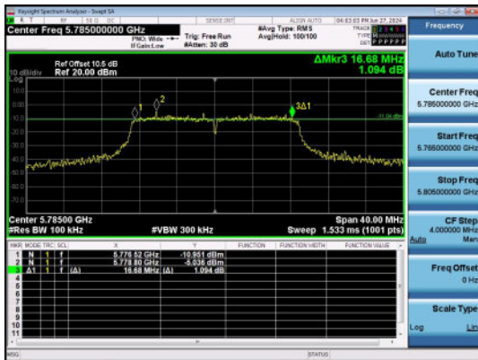
11N20SISO-Ant1-5785-PASS
