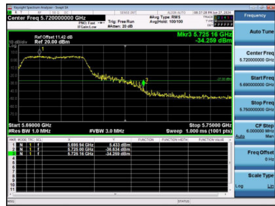
11A-Ant1-5700-PASS
