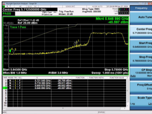
11AC40SISO-Ant1-5755-PASS
