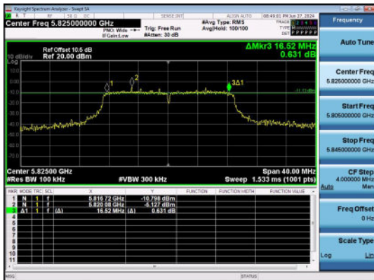
11AC20SISO-Ant1-5825-PASS
