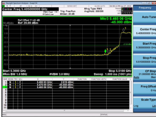
11AC20SISO-Ant1-5500-PASS
