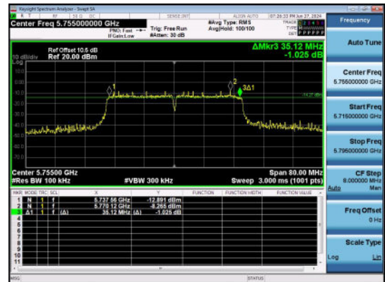
11AC40SISO-Ant1-5755-PASS
