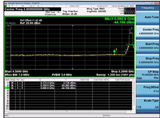
11N20SISO-Ant1-5180-PASS
