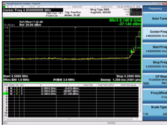
11N40SISO-Ant1-5190-PASS
