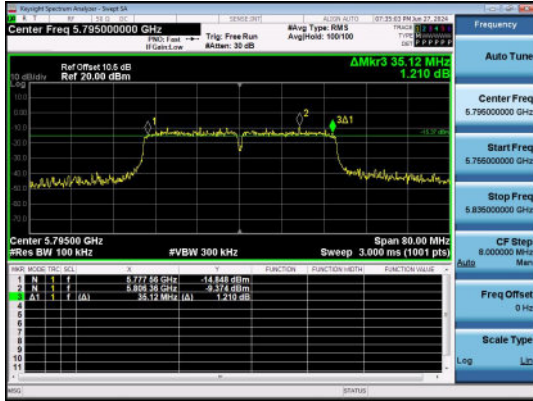
11AC40SISO-Ant1-5795-PASS
