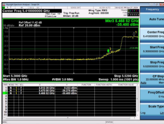
11N40SISO-Ant1-5510-PASS
