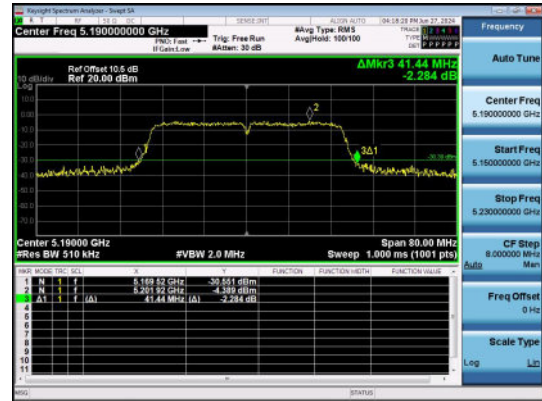
11N40SISO-Ant1-5190-26dB EBW
