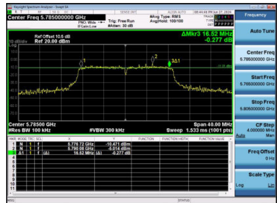
11AC20SISO-Ant1-5785-PASS
