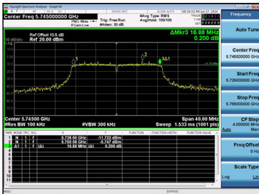
11AC20SISO-Ant1-5745-PASS
