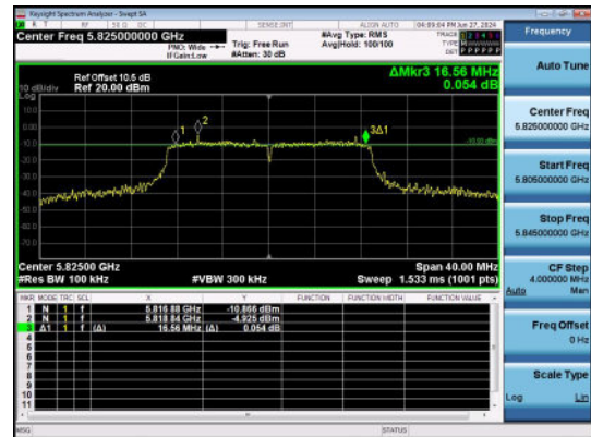
11N20SISO-Ant1-5825-PASS
