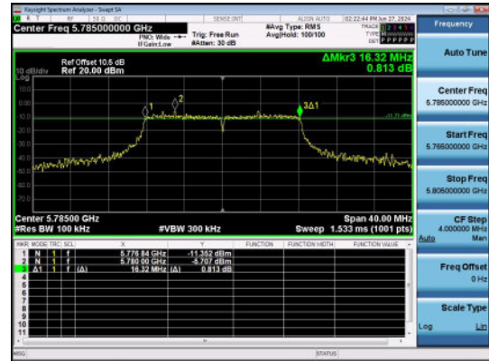
11A-Ant1-5785-PASS
