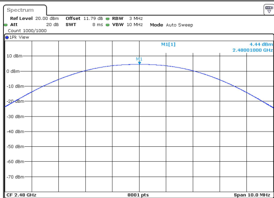
BLE_1M-Ant1-2480-PASS
