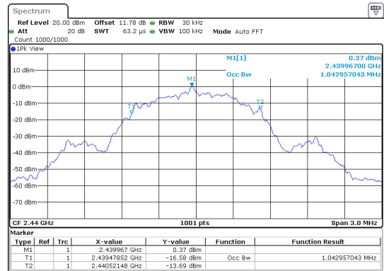
BLE_1M-Ant1-2440
