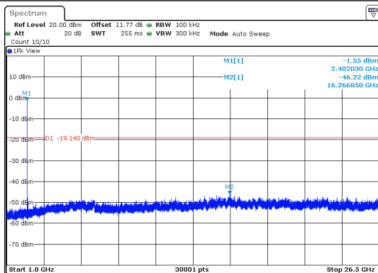
BLE_1M-Ant1-2402-1000~26500-PASS
