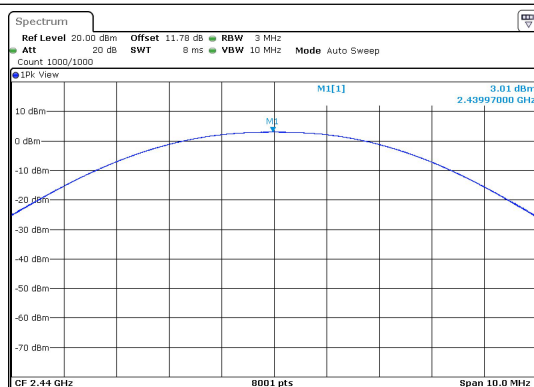
BLE_1M-Ant1-2440-PASS
