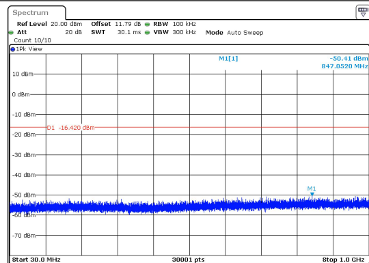
BLE_1M-Ant1-2480-30~1000-PASS
