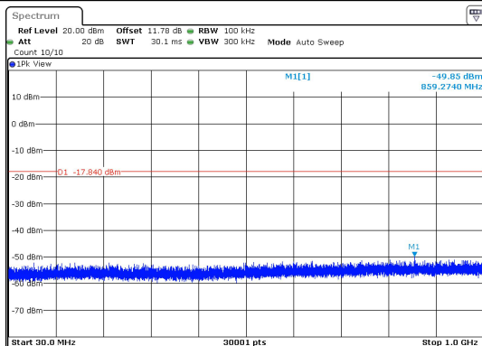
BLE_1M-Ant1-2440-30~1000-PASS
