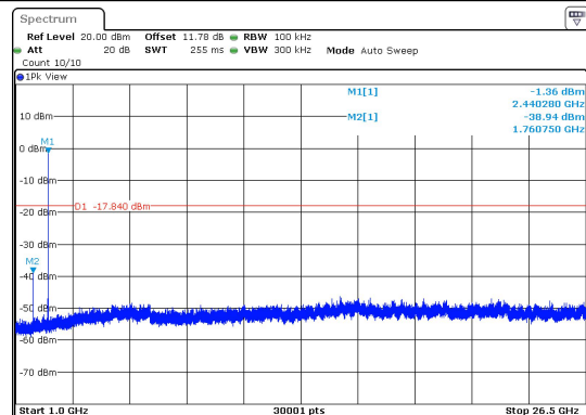
BLE_1M-Ant1-2440-1000~26500-PASS
