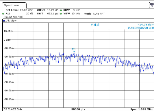
BLE_1M-Ant1-2402-PASS
