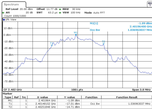
BLE_1M-Ant1-2402
