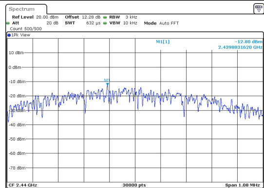
BLE_1M-Ant1-2440-PASS
