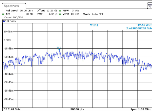
BLE_1M-Ant1-2480-PASS
