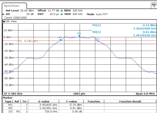
BLE_1M-Ant1-2402-PASS
