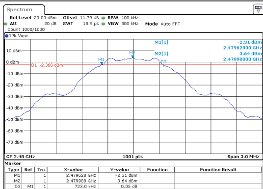
BLE_1M-Ant1-2480-PASS
