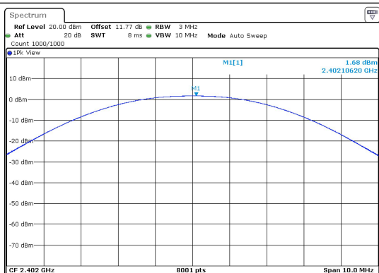
BLE_1M-Ant1-2402-PASS
