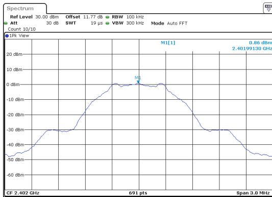
BLE_1M-Ant1-2402-0~Reference-PASS
