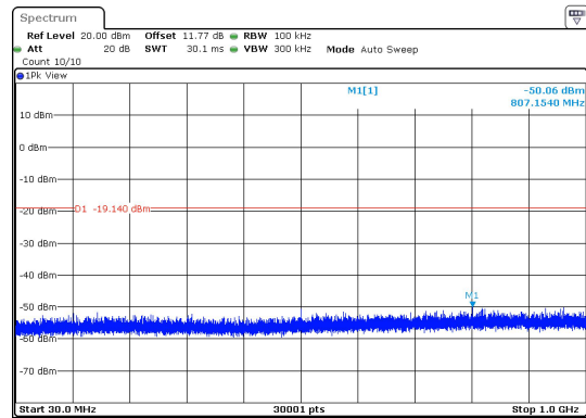
BLE_1M-Ant1-2402-30~1000-PASS
