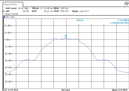
BLE_1M-Ant1-2440-0~Reference-PASS
