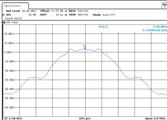
BLE_1M-Ant1-2480-0~Reference-PASS
