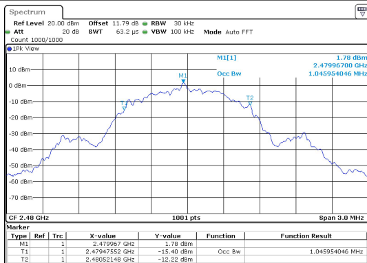
BLE_1M-Ant1-2480
