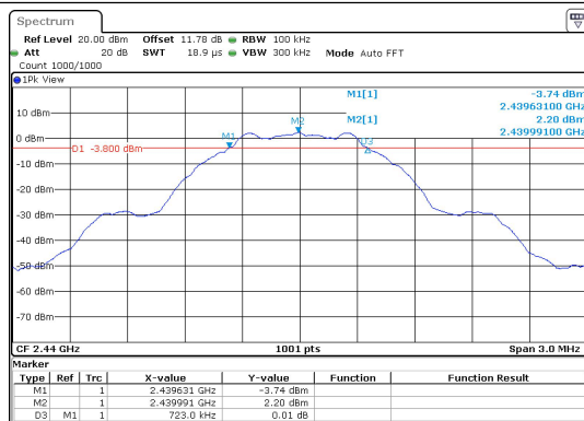
BLE_1M-Ant1-2440-PASS
