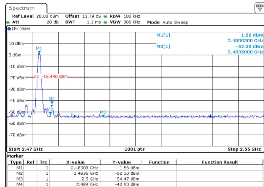
BLE_1M-Ant1-2480-PASS
