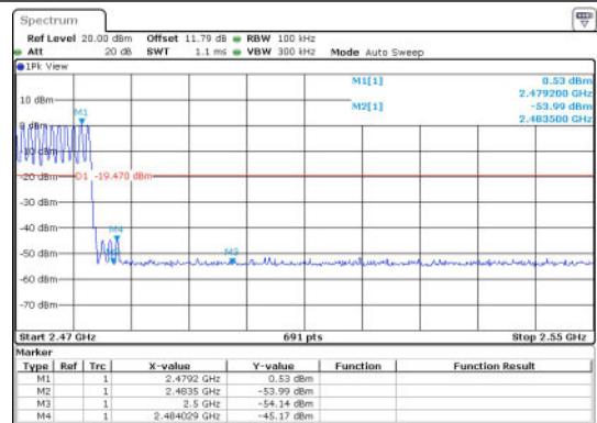
DH5-Ant1-Hop_2480-PASS
