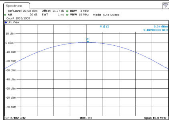
2DH5-Ant1-2402-PASS
