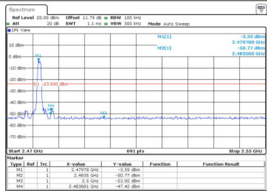
3DH5-Ant1-2480-PASS
