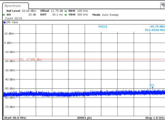
DH5-Ant1-2480-30~1000-PASS
