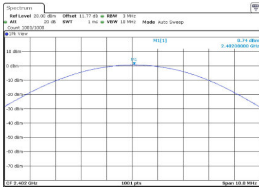
3DH5-Ant1-2402-PASS
