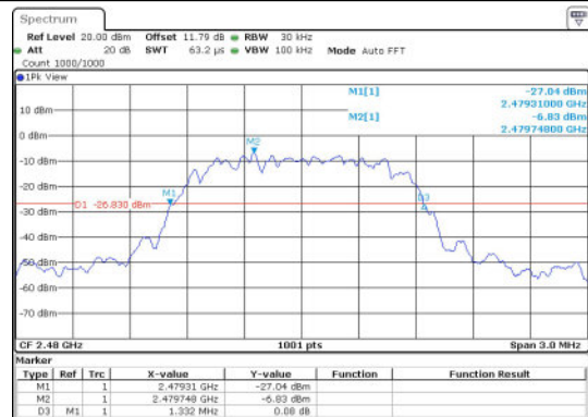
2DH5-Ant1-2480
