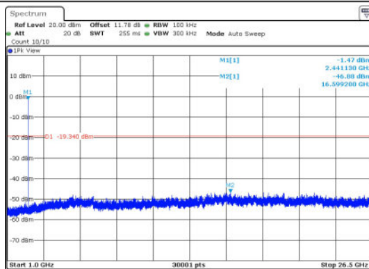
DH5-Ant1-2441-1000~26500-PASS
