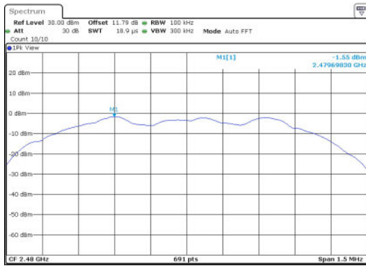
3DH5-Ant1-2480-0~Reference-PASS
