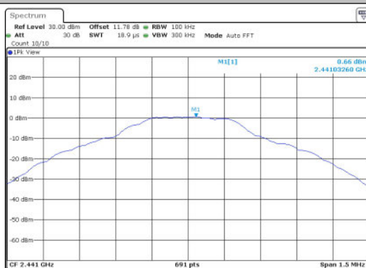
DH5-Ant1-2441-0~Reference-PASS
