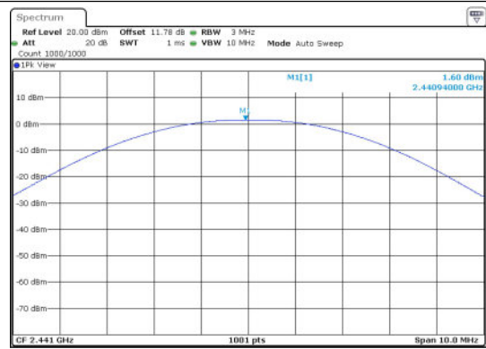
DH5-Ant1-2441-PASS
