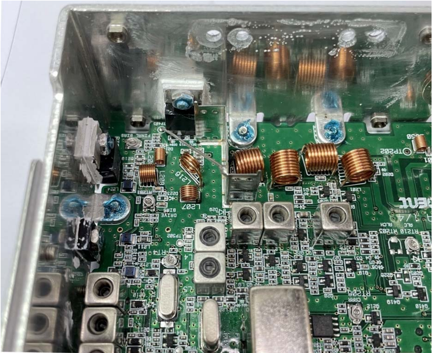
Figure E22.5 – Internal, Main PCB, WX Removed
