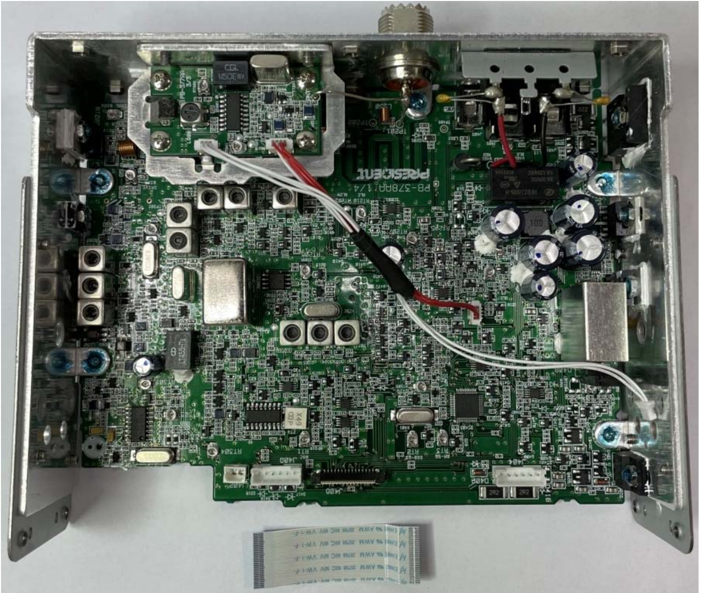
Figure E22.3 – Internal, Main PCB, Top
