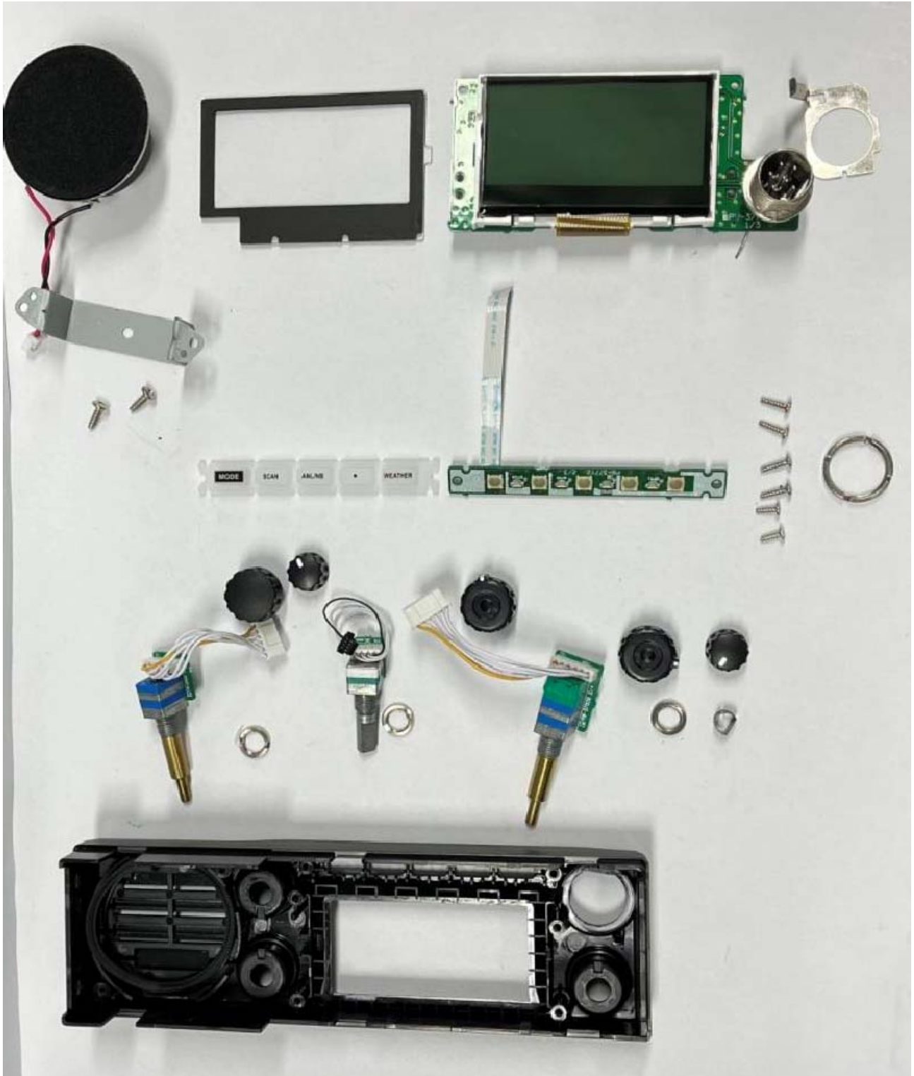
Figure E22.7 – Internal, Main PCB, Front Assembly Component
