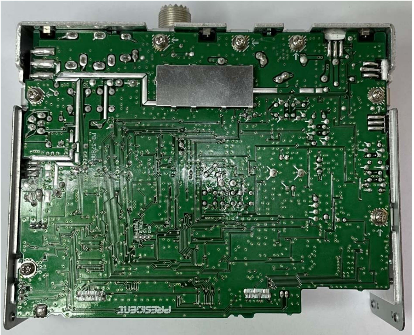
Figure E22.4 – Internal, Main PCB, Bottom
