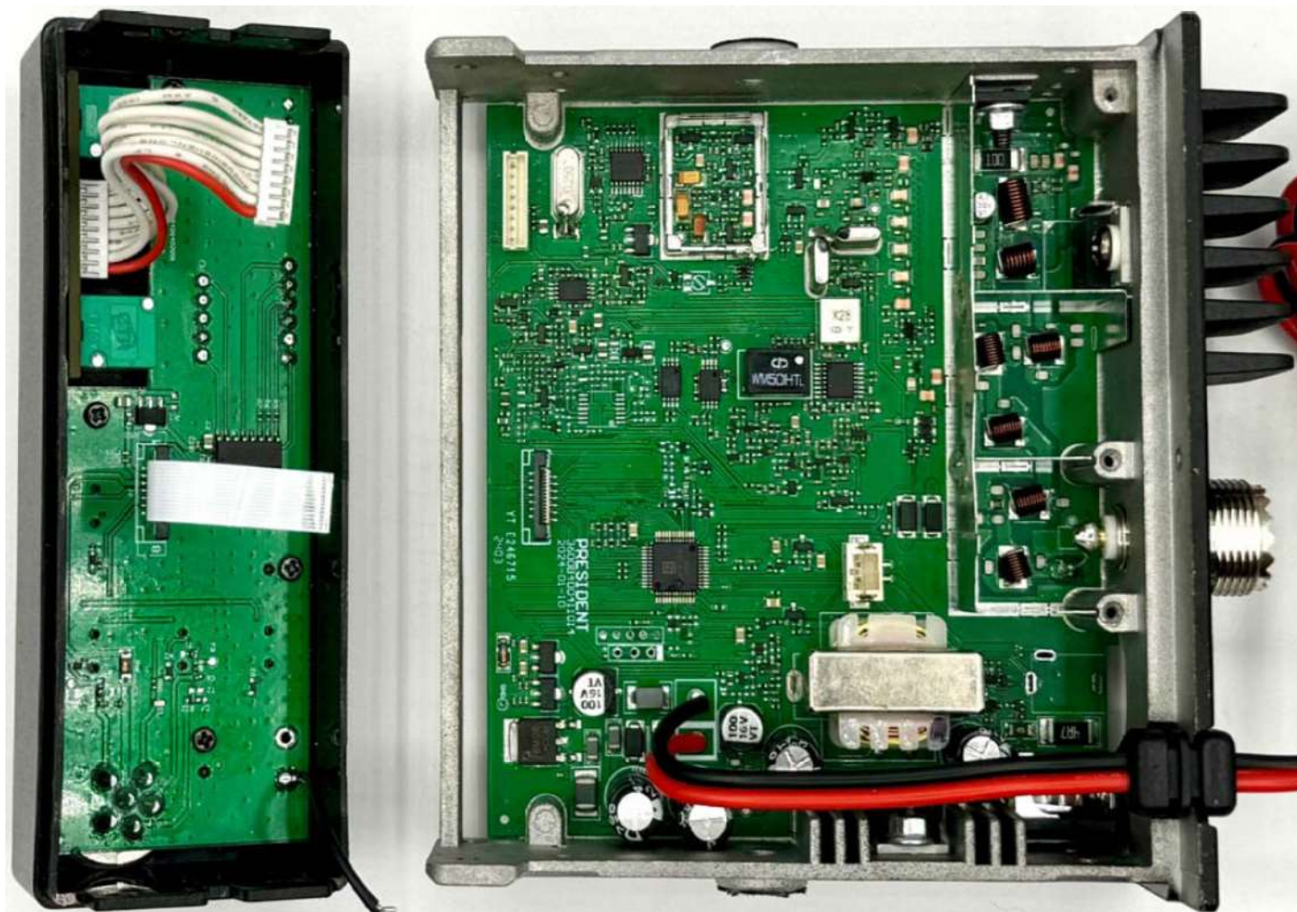
Figure E17.2 – Internal, Bottom/Front Cover Removed
