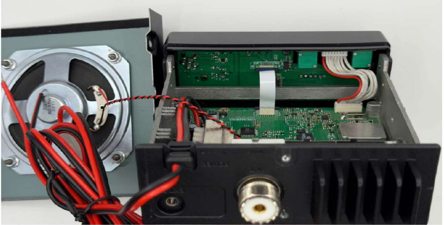
Figure E17.1 – Internal, Bottom Cover Removed
