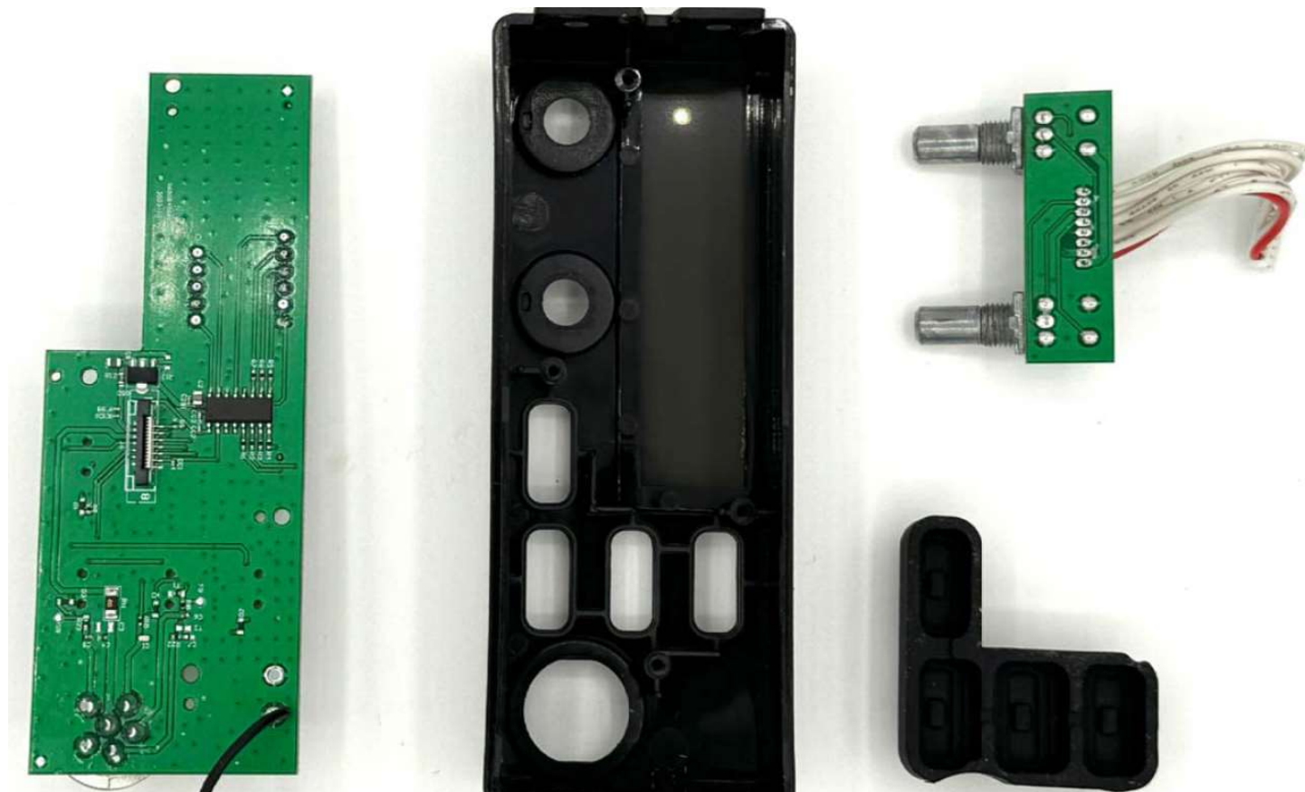
Figure E17.4 – Internal, Back Controls
