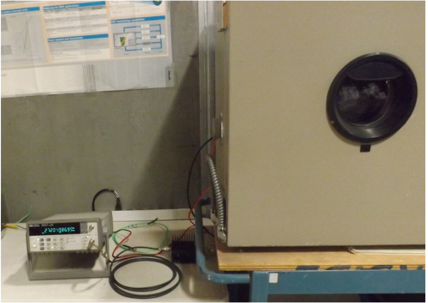
Figure E18.9 – Setup, Frequency Stability
