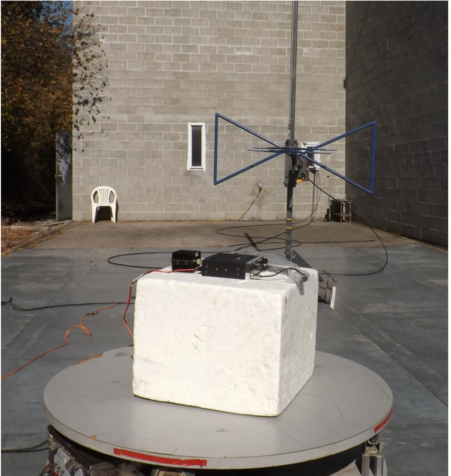
Figure E18.7 – Setup, Radiated Measurements, 30 - 1000MHz
