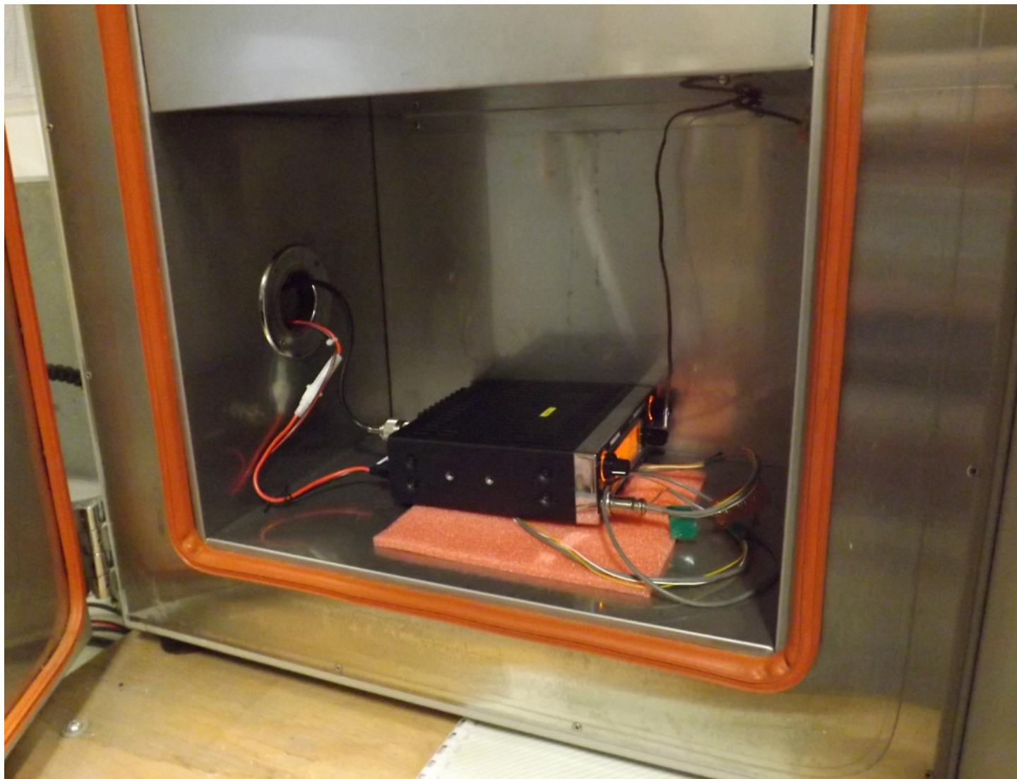
Figure E18.10 – Setup, Frequency Stability
