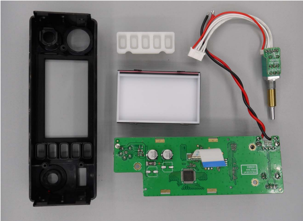
Figure E22.7 – Internal, Front Components
