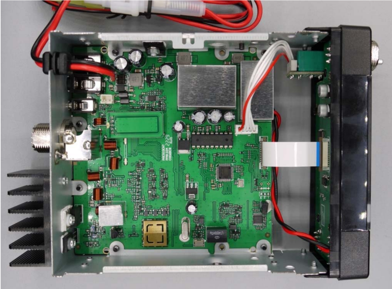
Figure E22.1 – Internal, Bottom Removed
