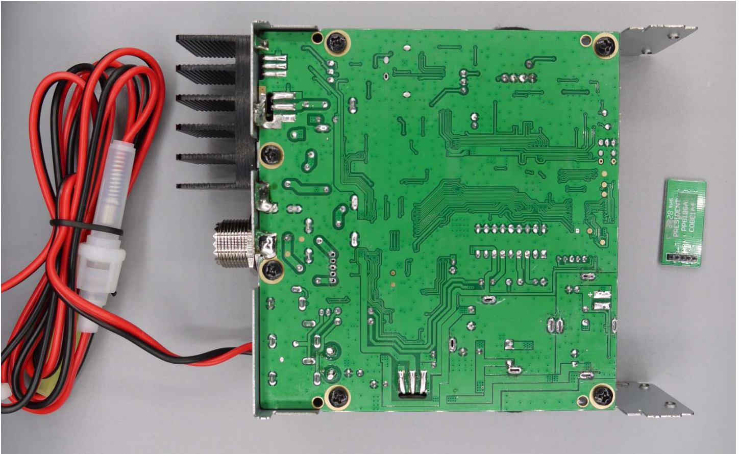
Figure E22.3 – Internal, Top Removed
