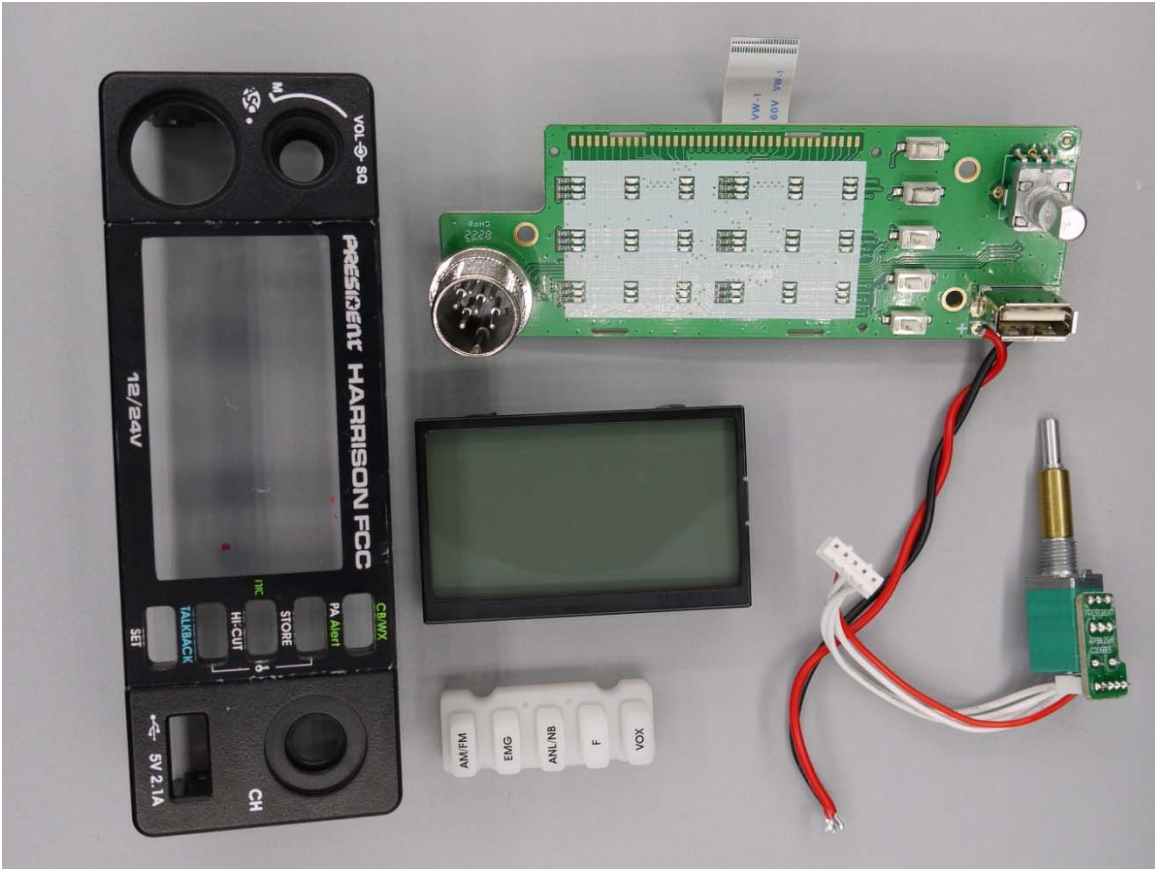
Figure E22.6 – Internal, Front Components
