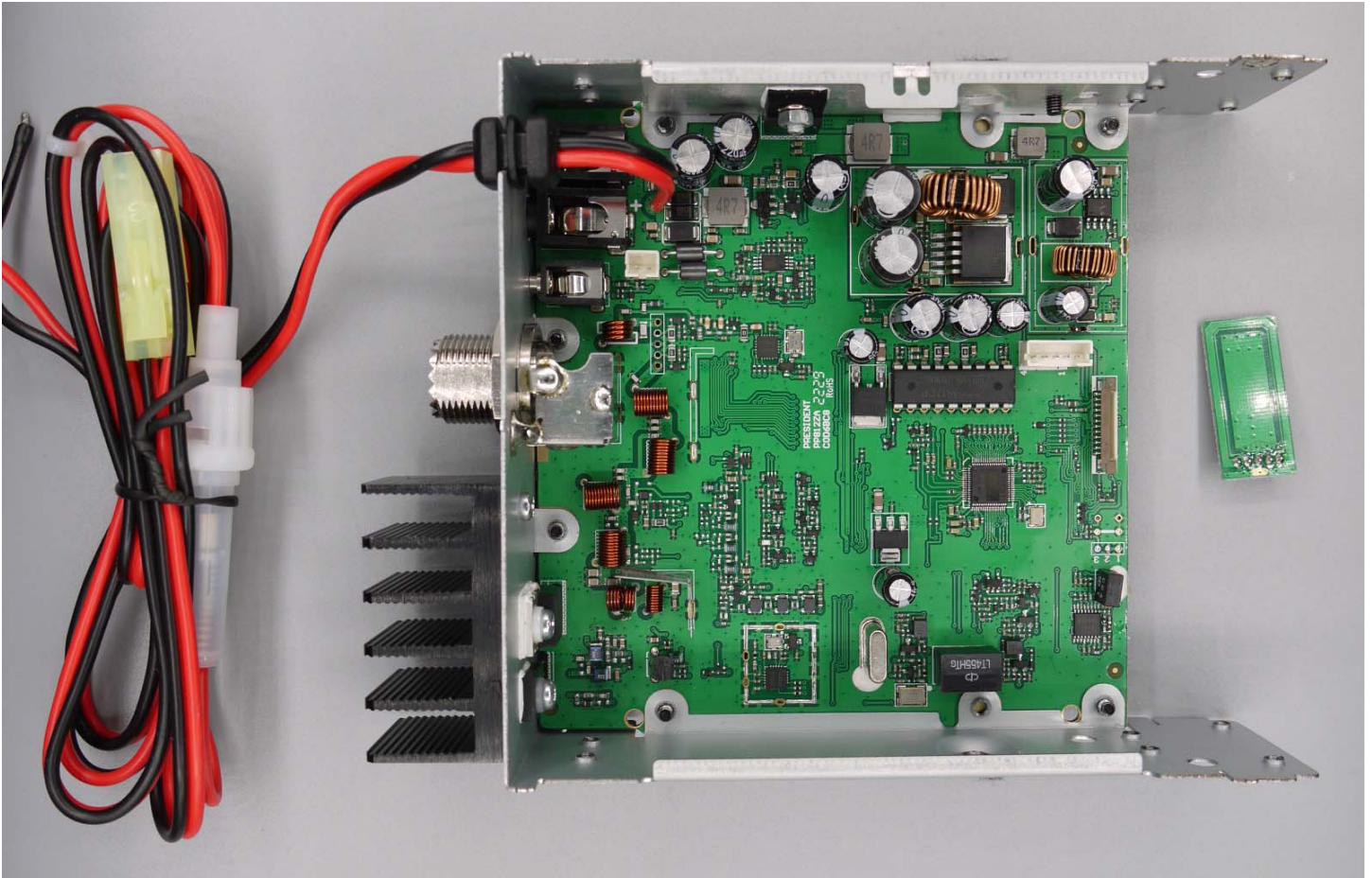
Figure E22.2 – Internal, Shields Removed
