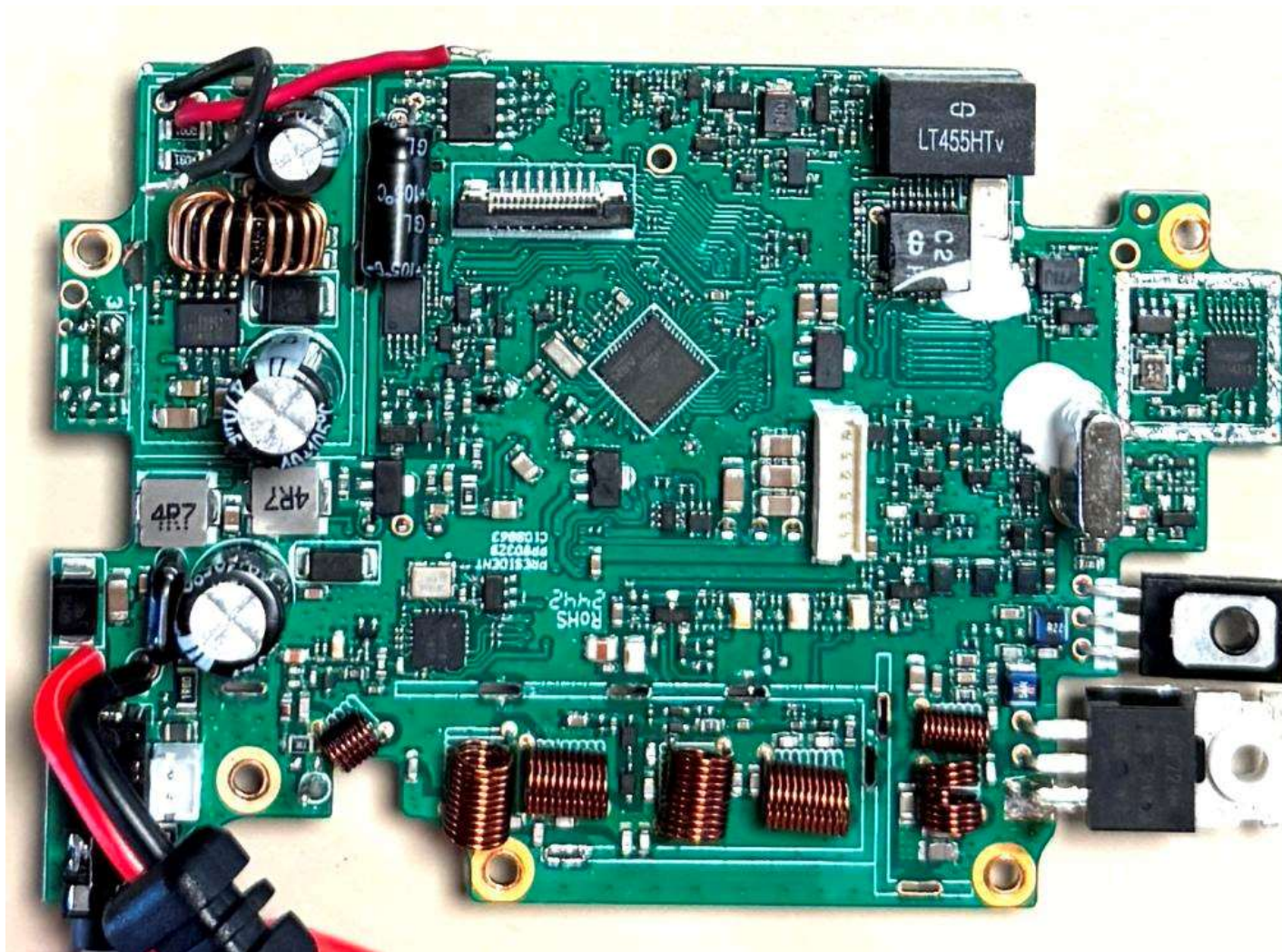
Figure E9.3 – Internal, Main PCB, Top
