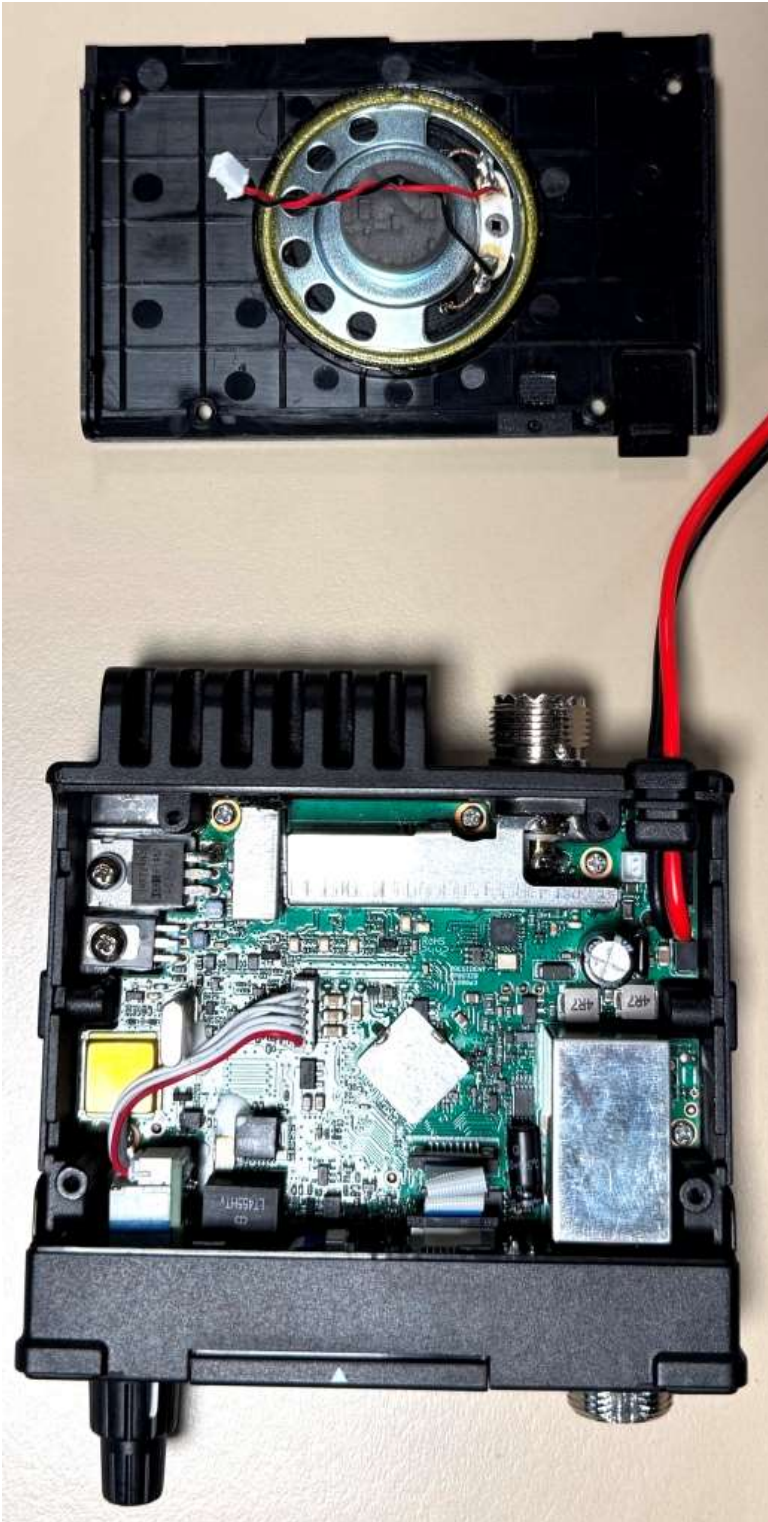
Figure E9.1 – Internal, Bottom Removed
