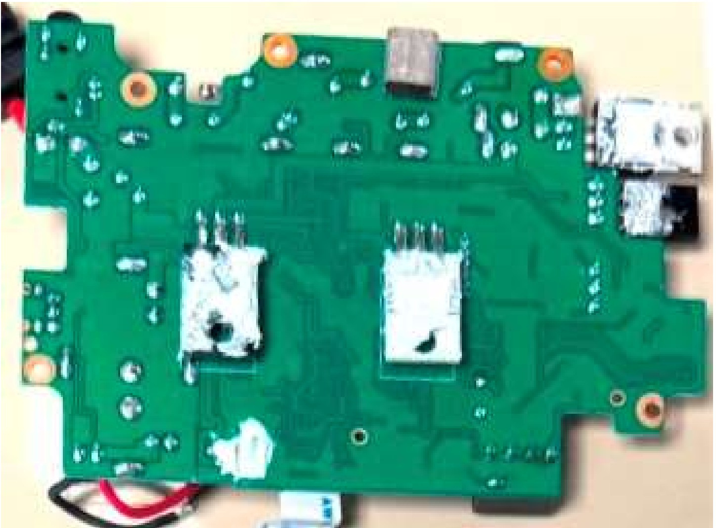
Figure E9.2 – Internal, Main PCB Bottom
