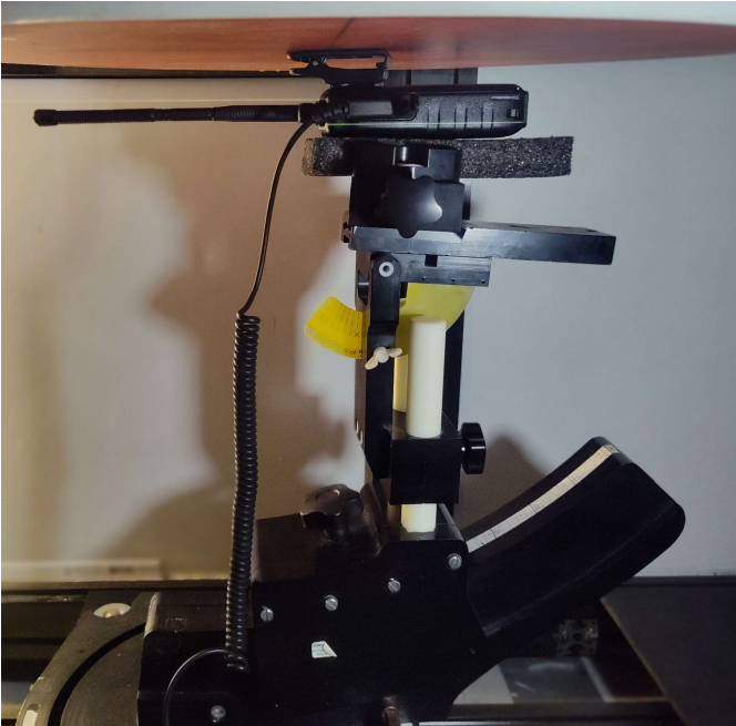
Figure C.1 – Setup Photo, Body – B1
