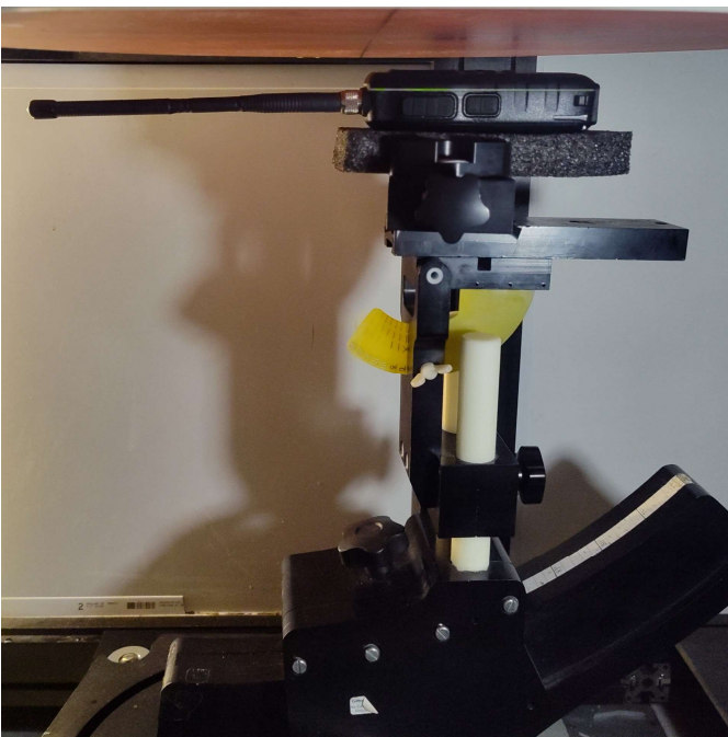
Figure C.2 – Setup Photo, Face -F1
