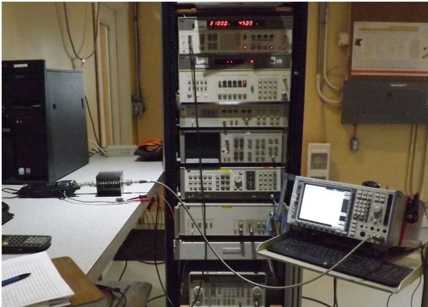
Figure E13.1 – Setup, Antenna Port Conducted
