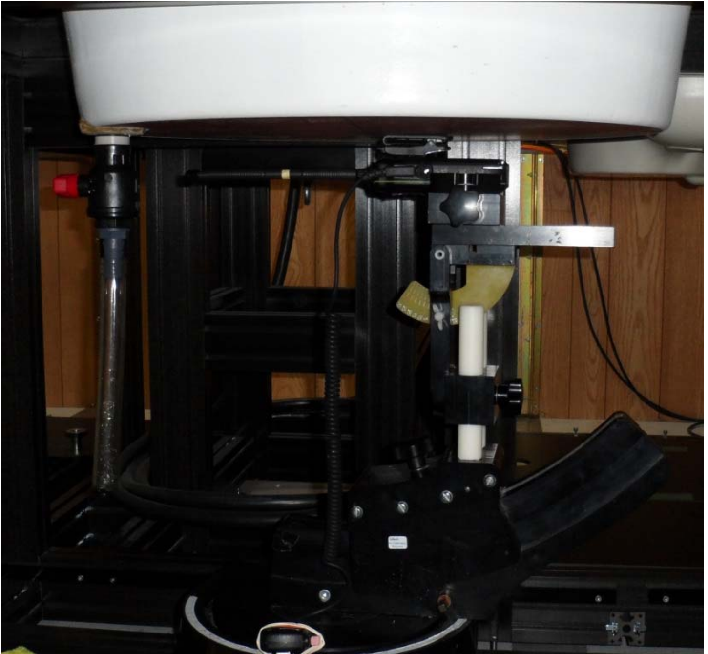
Figure E19.3 – Setup Photo – Body Configuration, Separation Distance: 0mm
