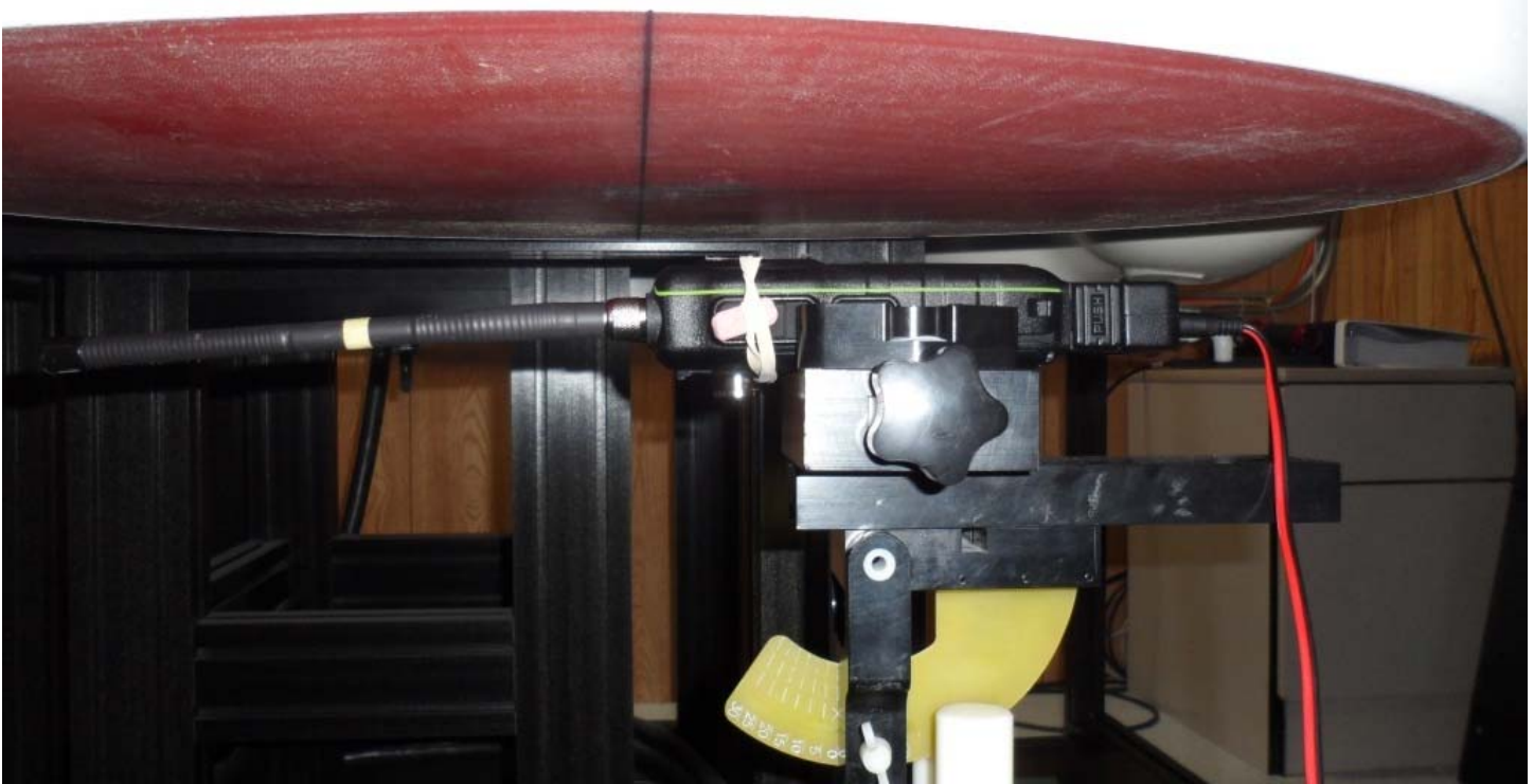
Figure E19.6 – Setup Photo – Face Configuration w/ Automotive Adapter, Enlarged, Separation Distance: 20mm
