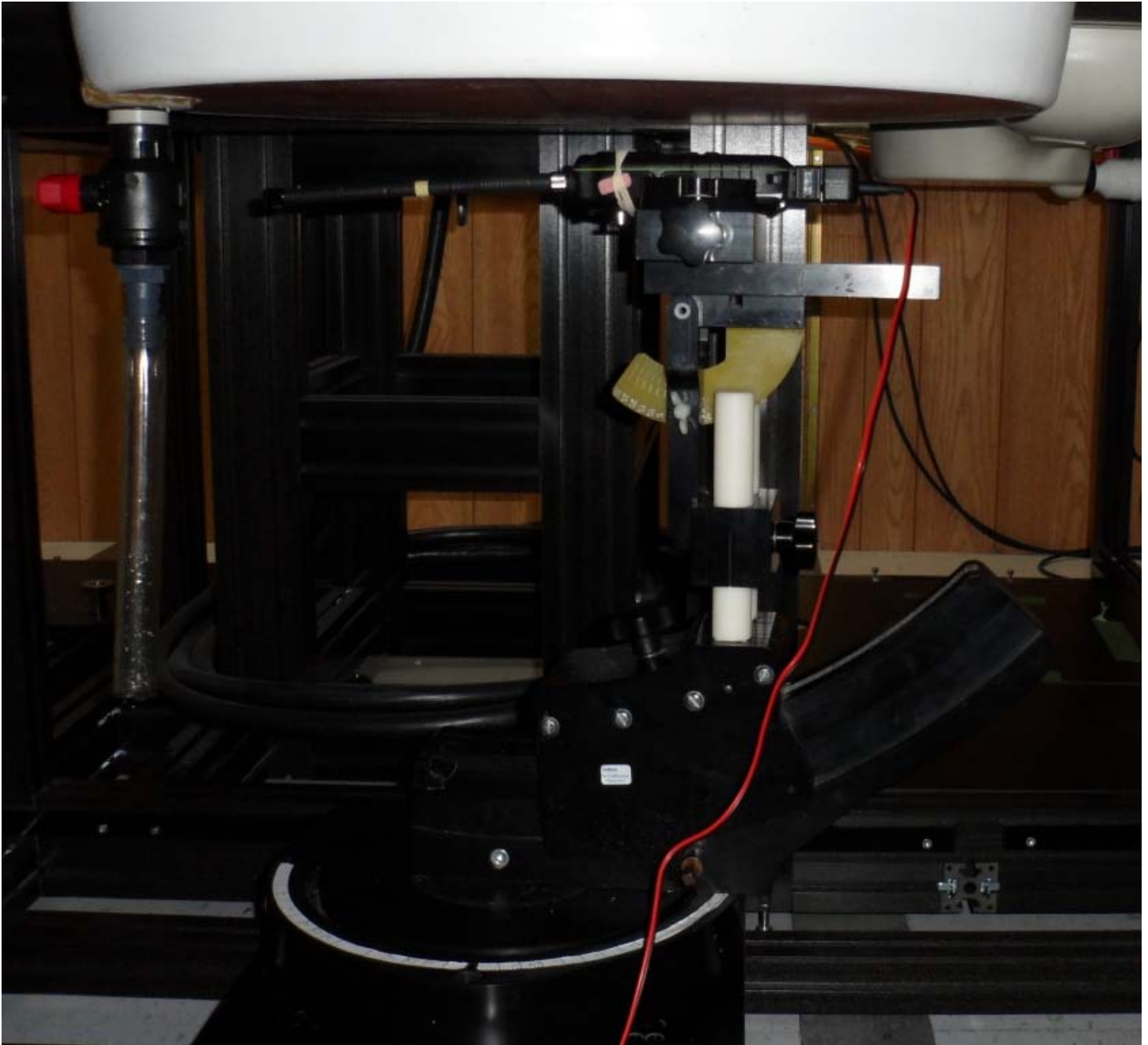
Figure E19.5 – Setup Photo – Face Configuration w/ Automotive Adapter, Separation Distance: 20mm
