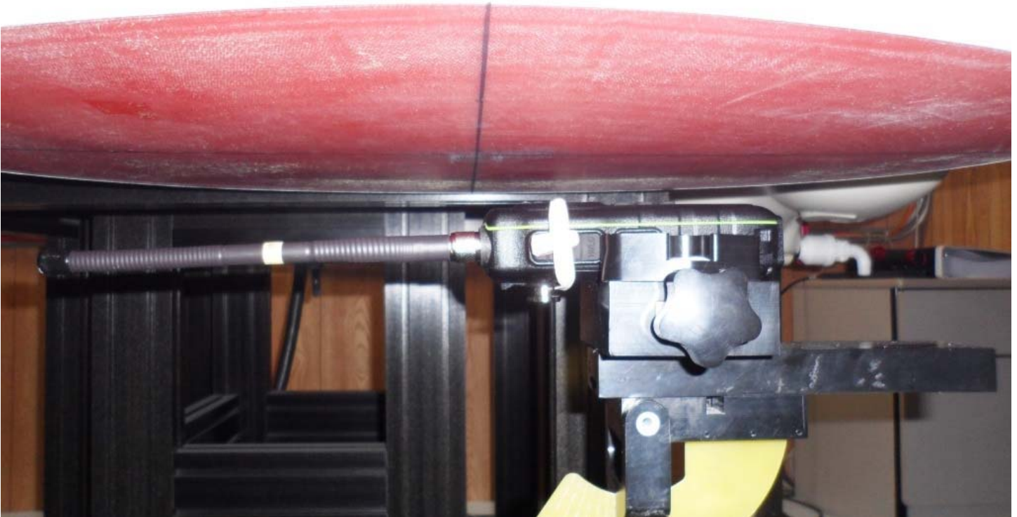
Figure E19.2 – Setup Photo – Face Configuration, Enlarged, DUT Separation Distance: 25mm
