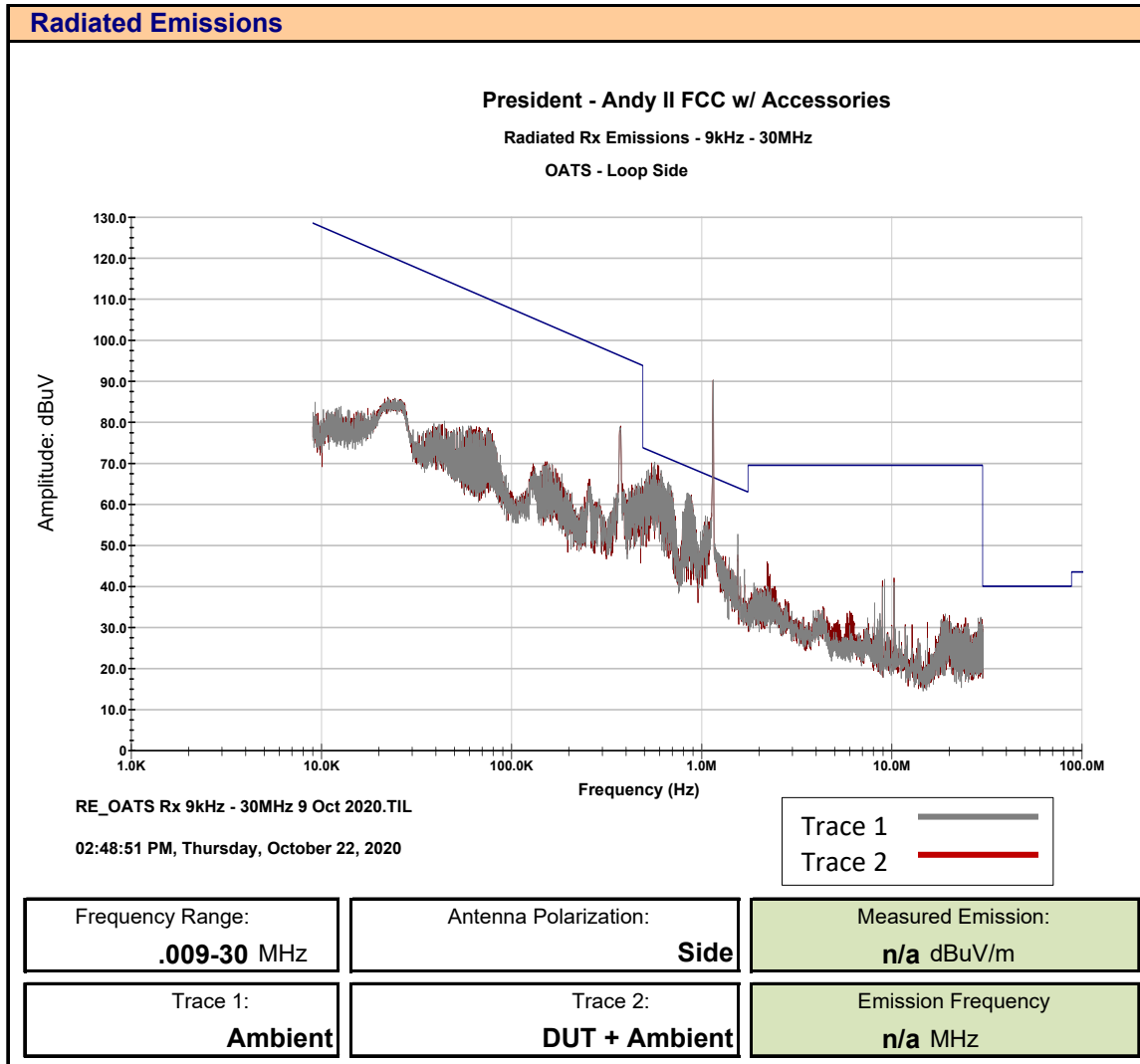
Plot 12.4 – Receiver Radiated Emissions, 9kHz – 30MHz, Side with Accessories
