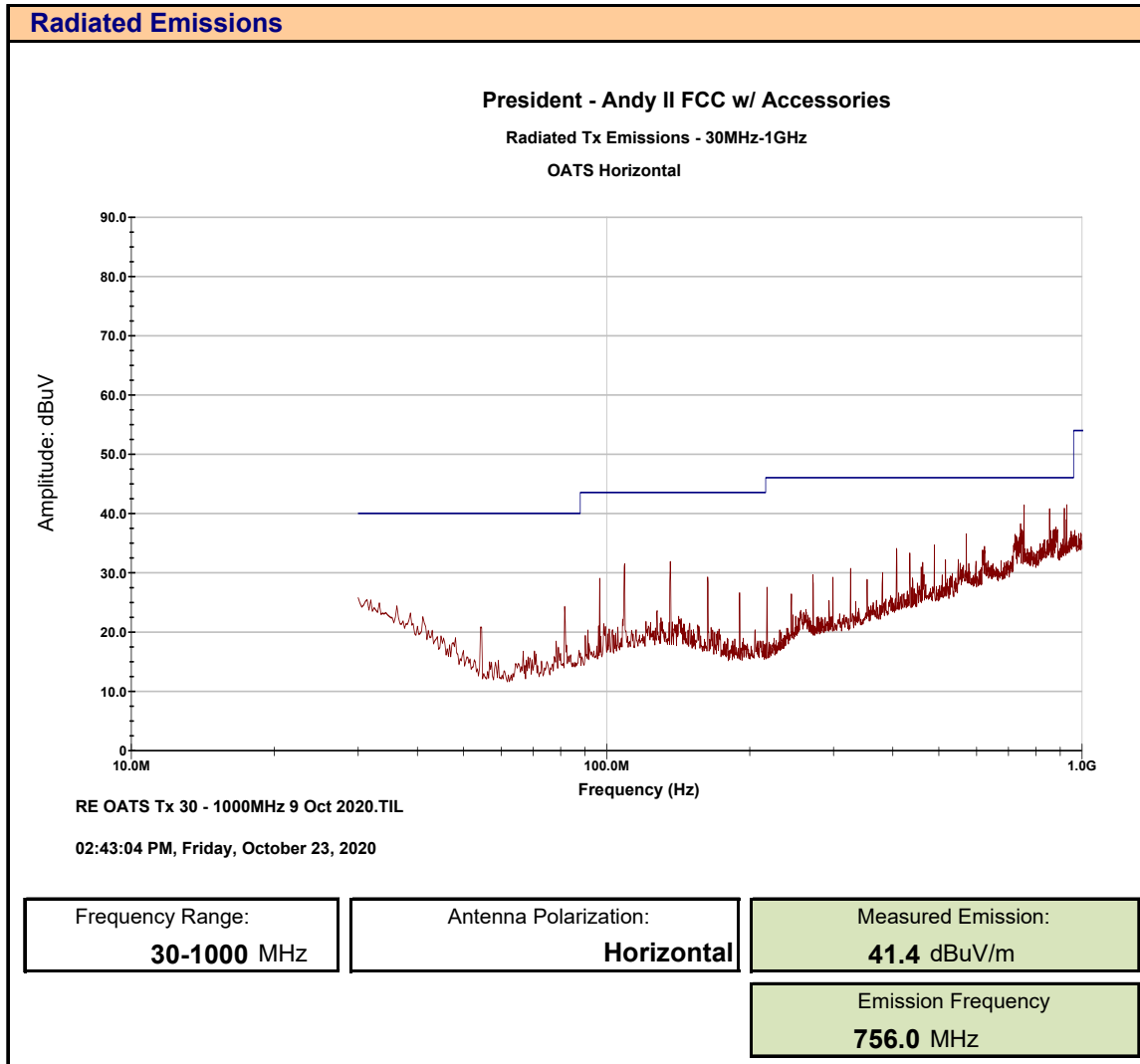
Plot 11.6 – Radiated Spurious Emissions OATS, 30MHz – 1000MHz, Horizontal with Accessories
