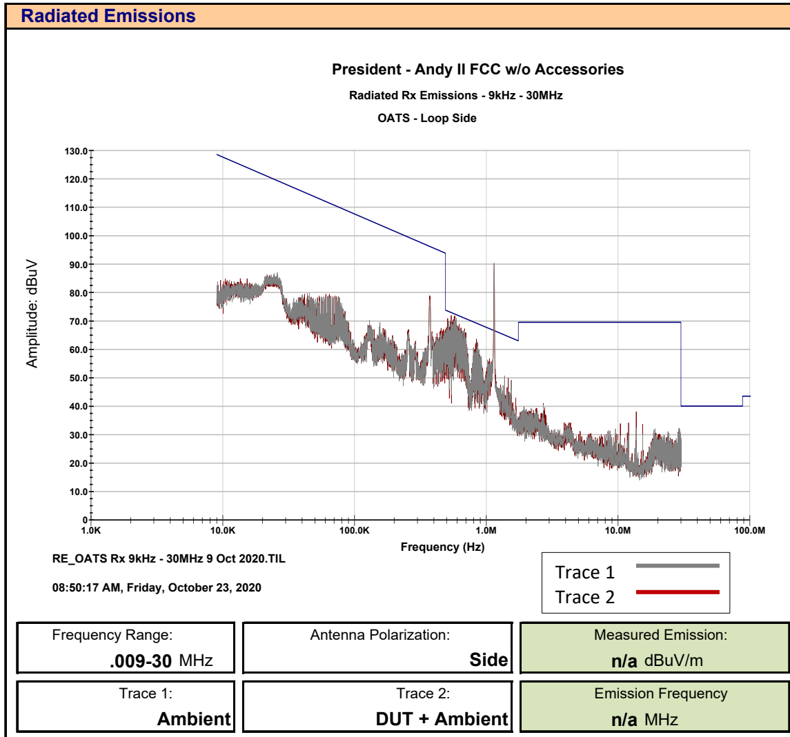
Plot 12.3 – Receiver Radiated Emissions, 9kHz – 30MHz, Side without Accessories
