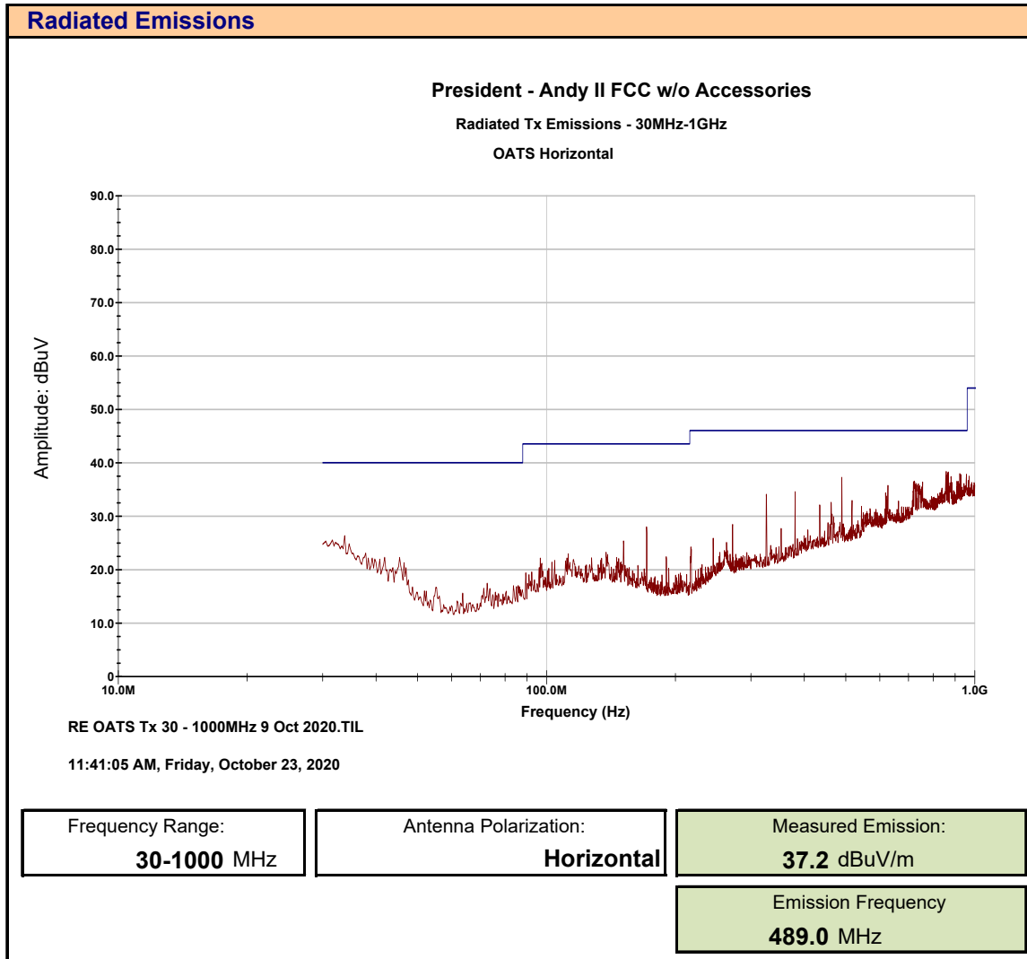
Plot 11.5 – Radiated Spurious Emissions OATS, 30MHz – 1000MHz, Horizontal without Accessories
