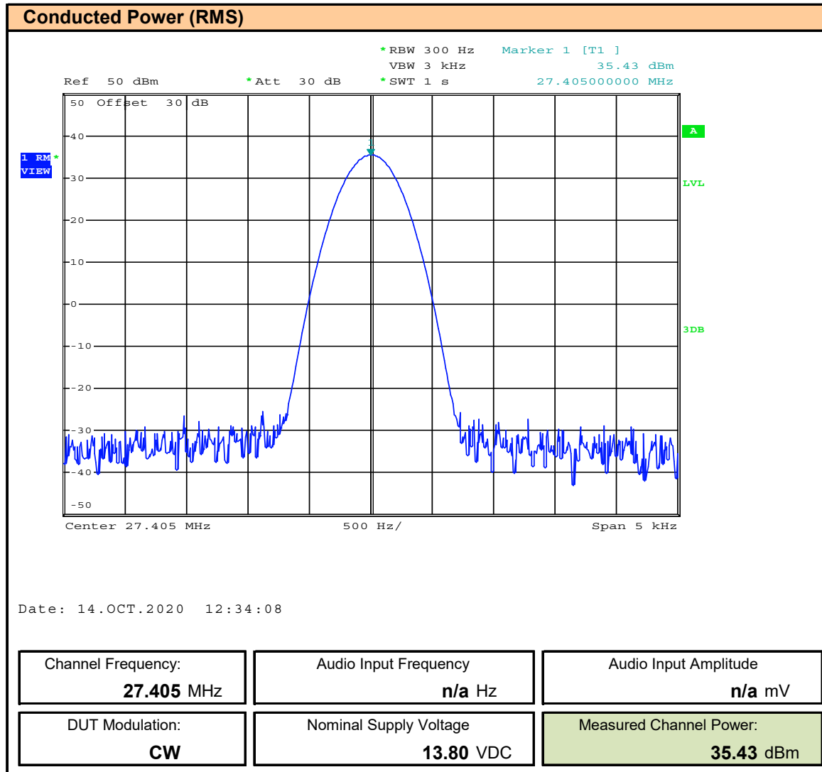
Plot 7.3 – Conducted Output Power – Channel 40
