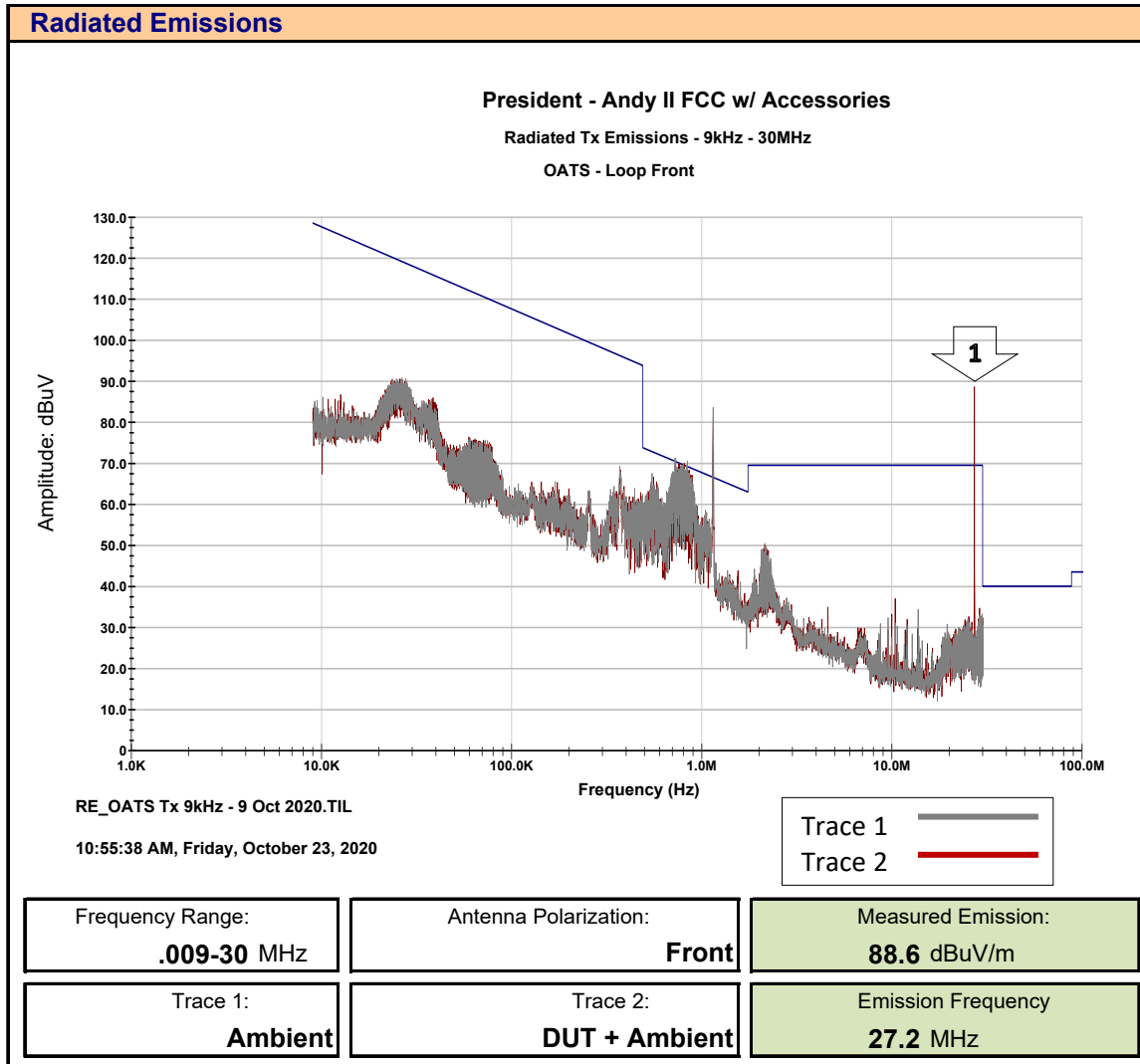
Plot 11.2 – Radiated Spurious Emissions OATS, 9kHz - 30MHz, Front with Accessories
