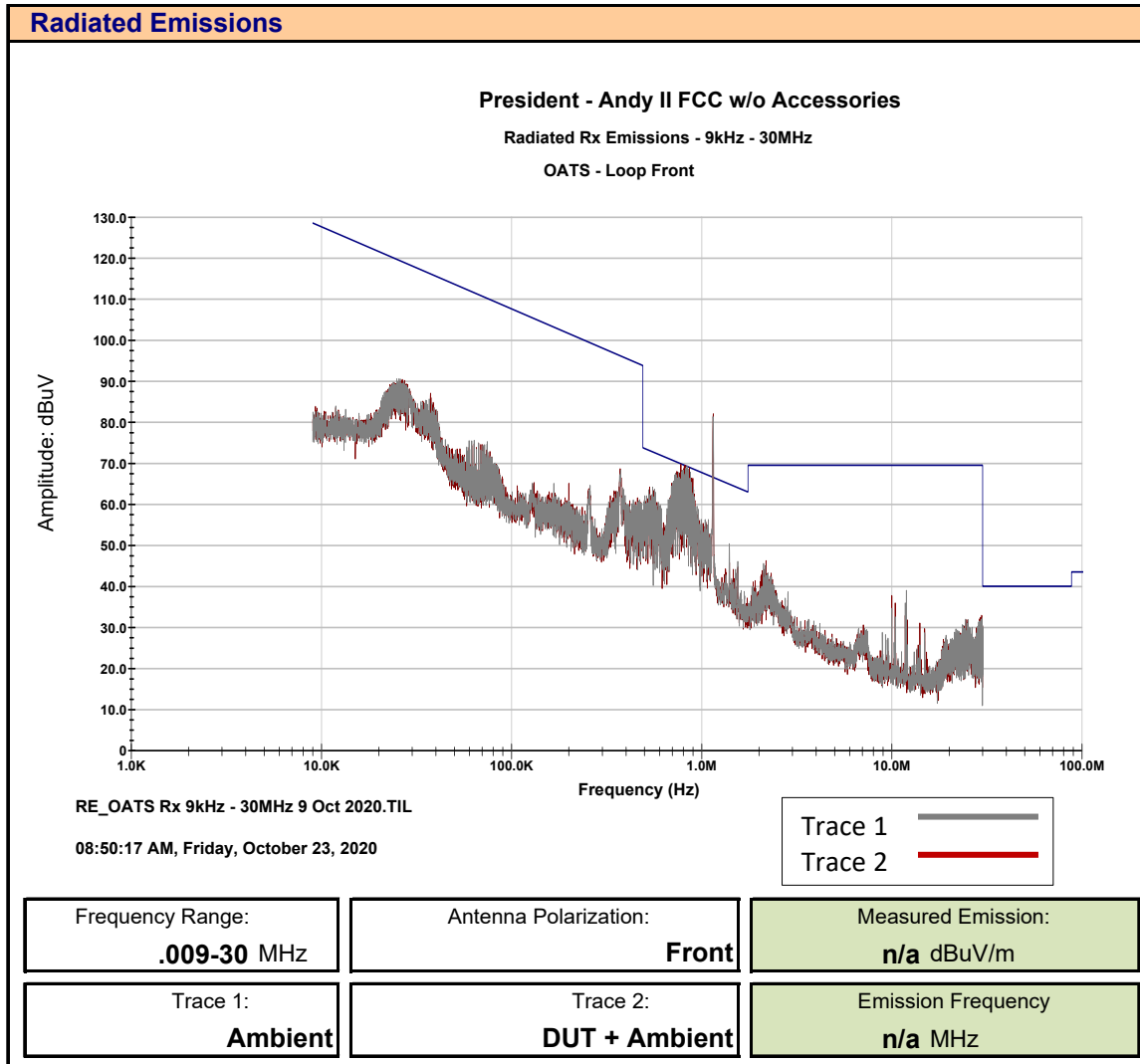
Plot 12.1 – Receiver Radiated Emissions, 9kHz – 30MHz, Front without Accessories
