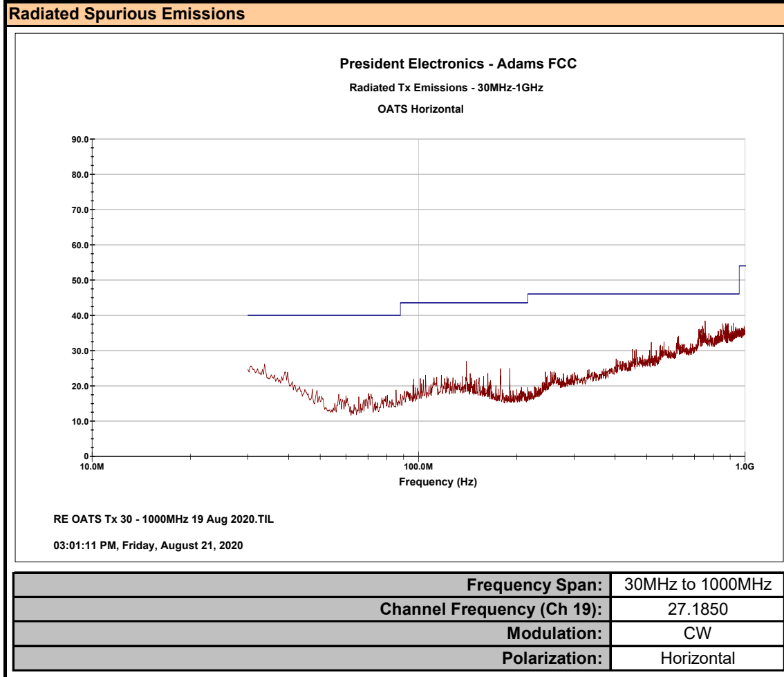
Plot 11.3 – Radiated Spurious Emissions, 30MHz – 1000MHz, Horizontal
