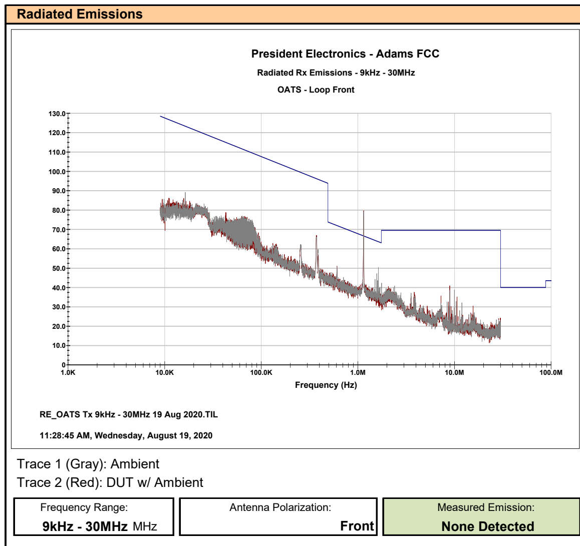
Plot 12.1 – Receiver Radiated Emissions 9kHz – 30MHz, Front
