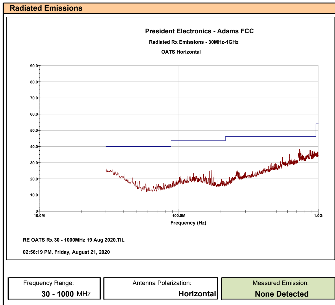
Plot 12.3 – Receiver Radiated Emissions, 30MHz - 1000MHz, Horizontal
