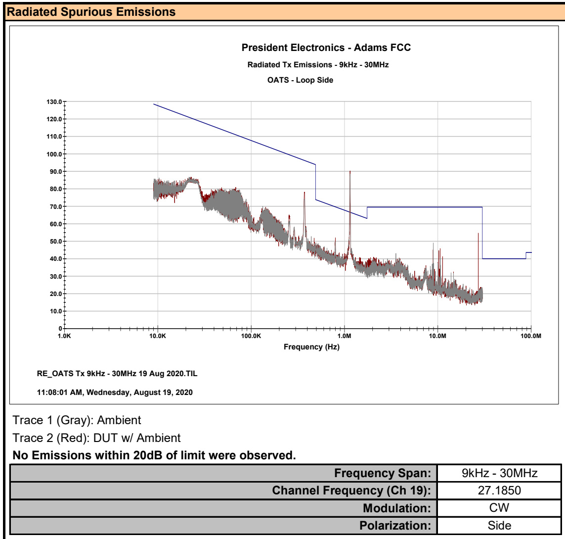
Plot 11.2 – Radiated Spurious Emissions 9kHz – 30MHz, Side
