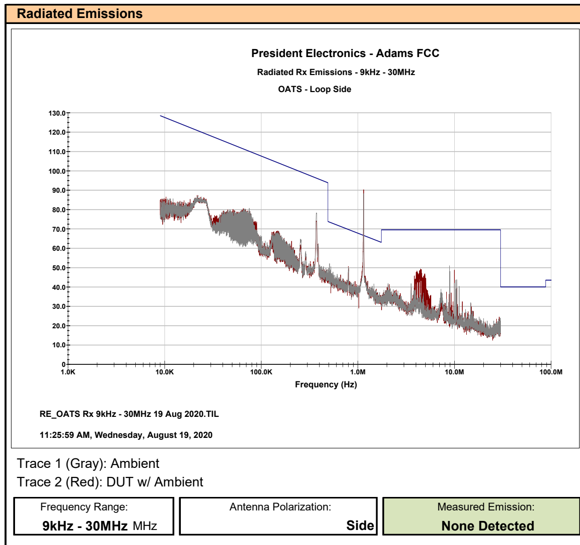
Plot 12.2 – Receiver Radiated Emissions 9kHz – 30MHz, Side
