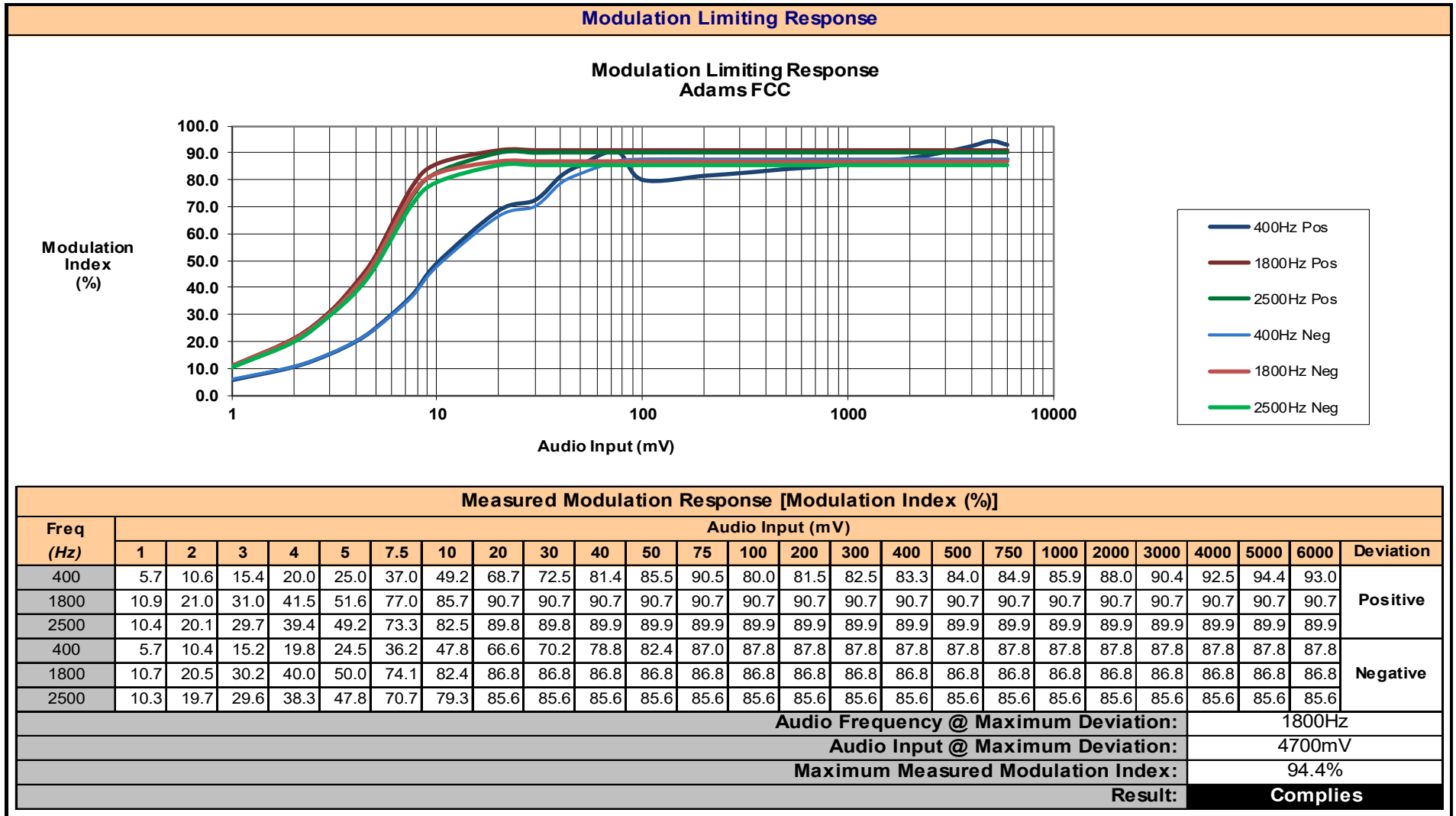
Plot 8.2 – Modulation Limiting Response
