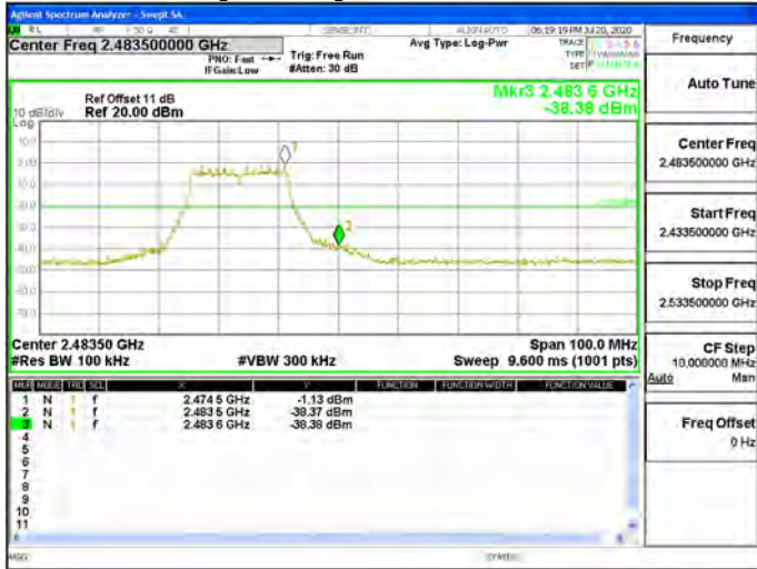
Band Edge_802.11g_20MHz_Chain0_2472MHz
