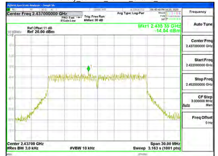
Power Density_802.11n_20MHz_Chain0_2437MHz
