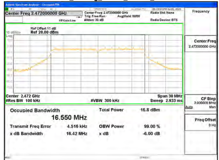
OBW 6dB_802.11g_20MHz_Chain0_2472MHz
