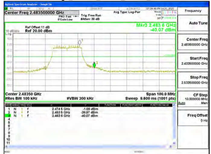
Band Edge_802.11n_20MHz_Chain0_2472MHz
