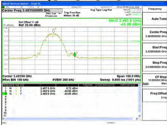
Band Edge_802.11b_20MHz_Chain0_2467MHz
