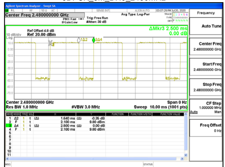
8DPSK_3M_DH3_2480MHz
