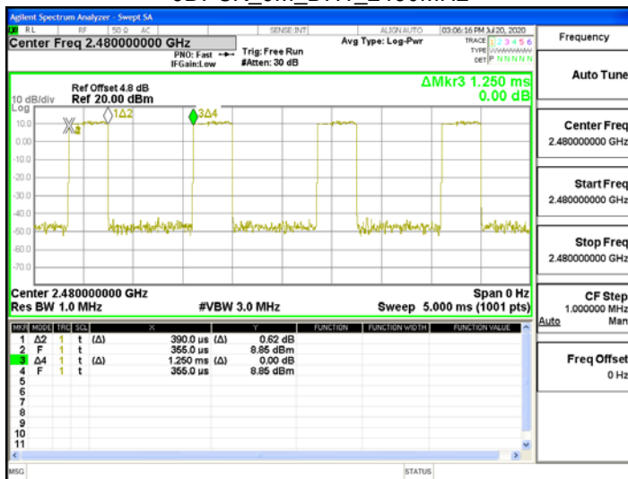
8DPSK_3M_DH1_2480MHz
