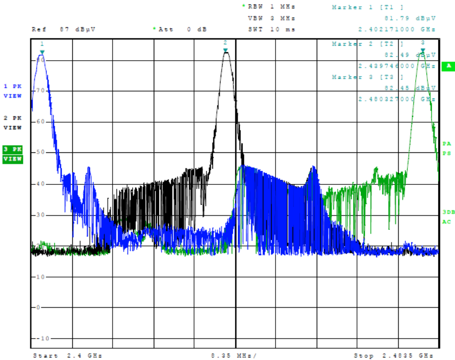
Figure 3 Plot of Transmitter Emissions (In 2402-2480 MHz Band)
