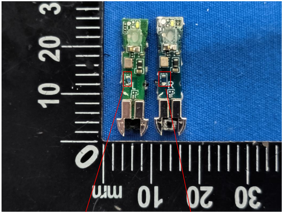
BT Antenna
