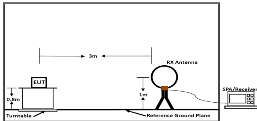
Below 30MHz
