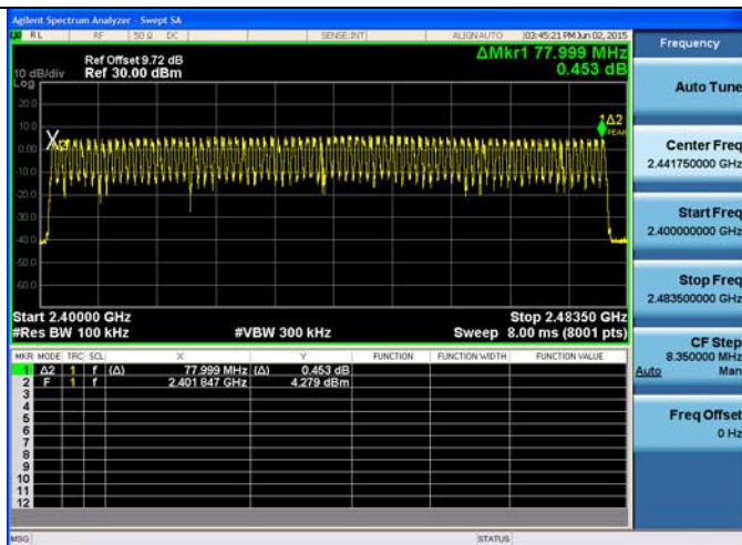
GFSK Modulation
