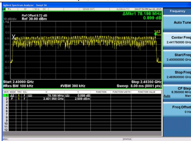
8DPSK Modulation
