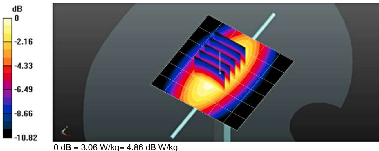
System Performance Check 835MHz Head 250mW
