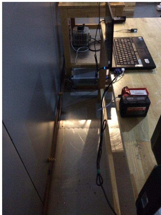
Conducted Emission test setup
