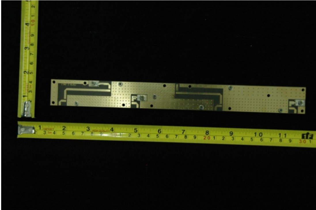
Splitter Top View
