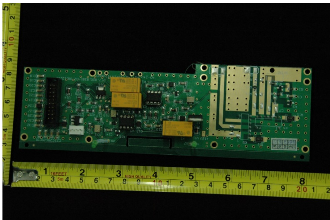
Switch board Top View
