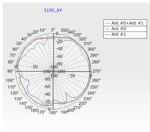
Phi_5150MHz
