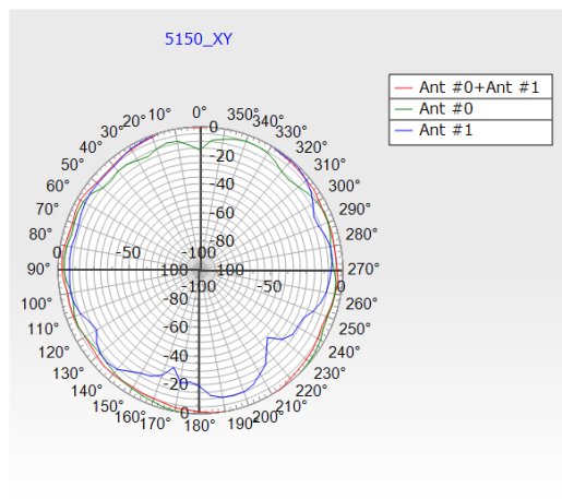
Theta_5150MHz
