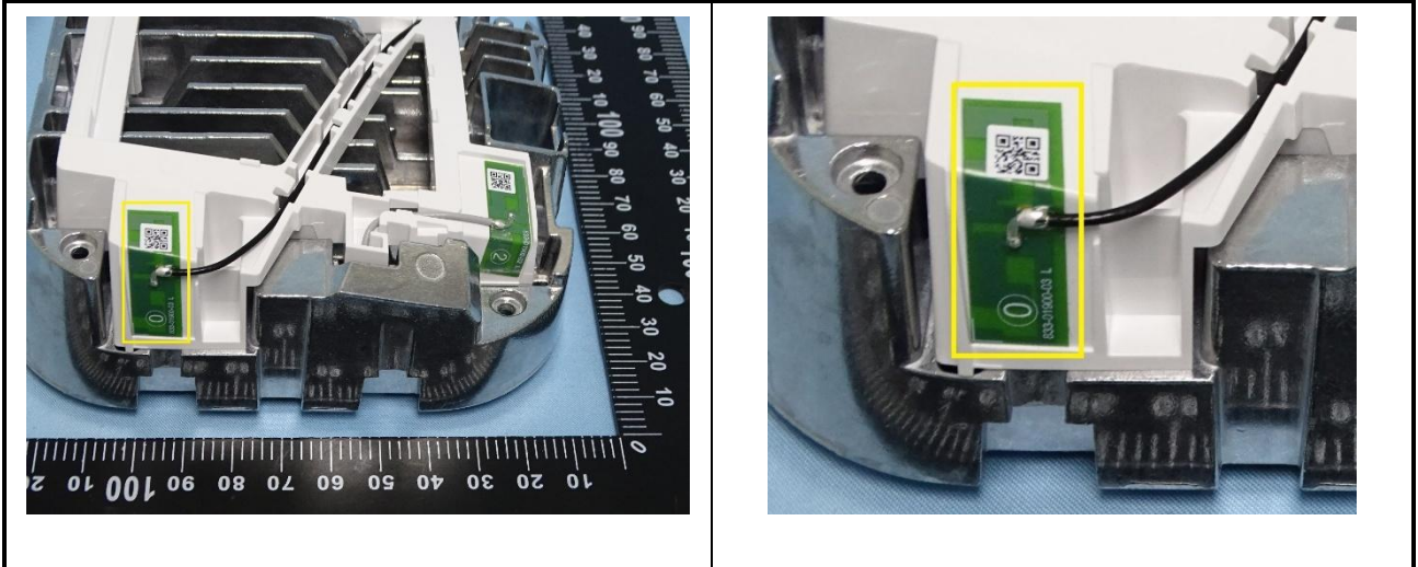
Fig.1 Antenna #0 (WLAN 2.4GHz/5GHz)
