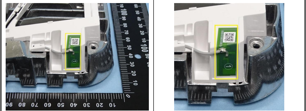
Fig.2 Antenna #1 (WLAN 2.4GHz/5GHz)
