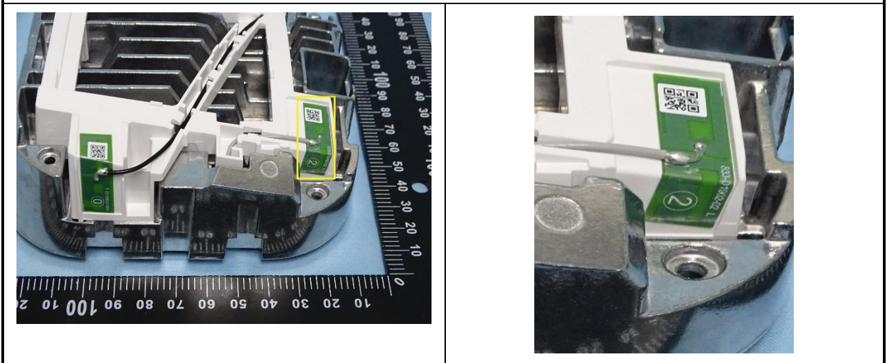
Fig.3 Antenna #2 (Bluetooth & ZigBee)
