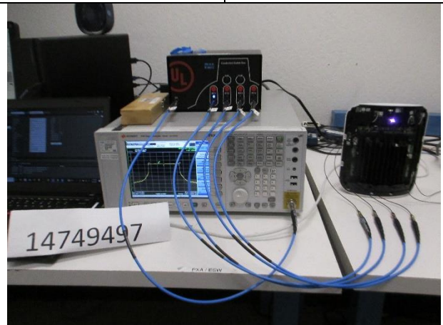
RF ANTENNA PORT CONDUCTED 5GHz UNII
