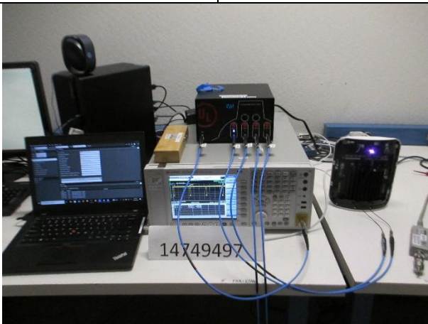
RF ANTENNA PORT CONDUCTED 2.4G DTS
