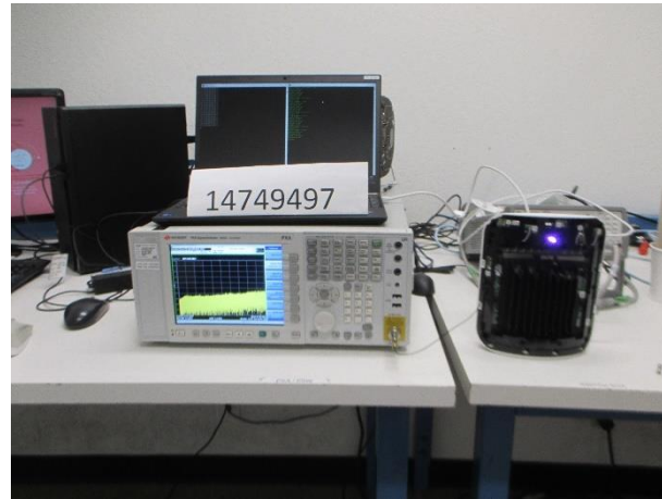
RF ANTENNA PORT CONDUCTED BLE/802.15.4
