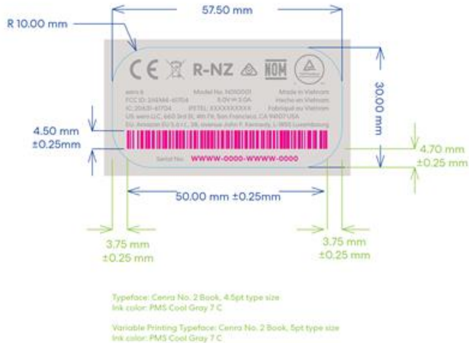
Figure 2: Model N010001 label dimension
