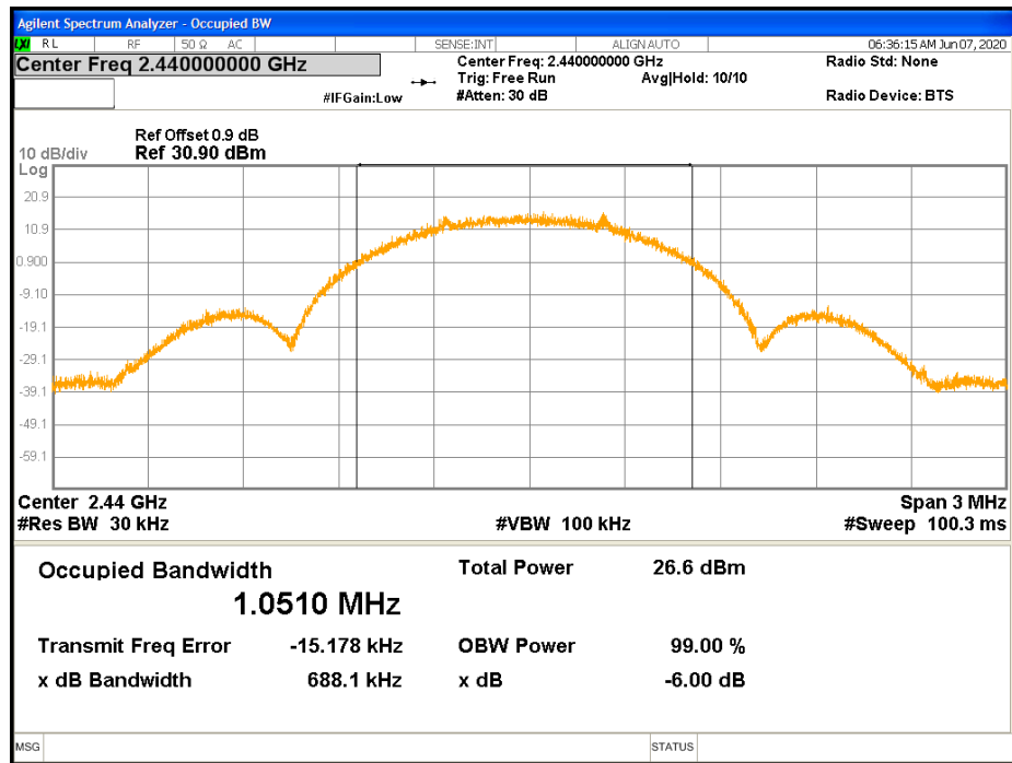
Figure 9: 99% Bandwidth-Transmitter -2440 MHz
