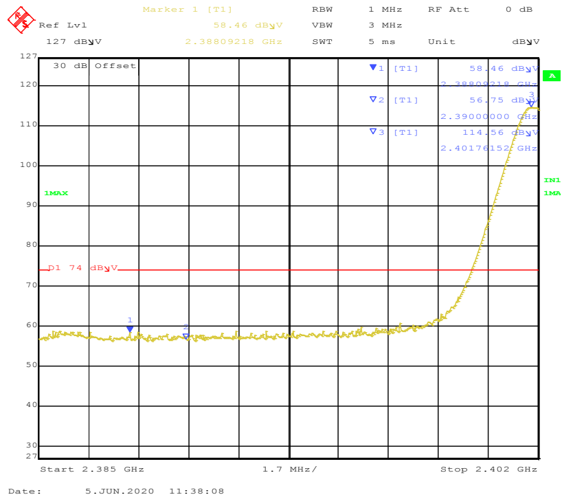
Figure 20: Band-edge-2402 MHz-V-Pk
