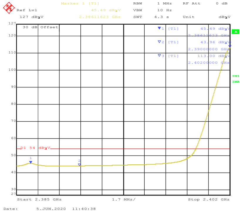
Figure 21: Band-edge-2402 MHz-V-Avg
