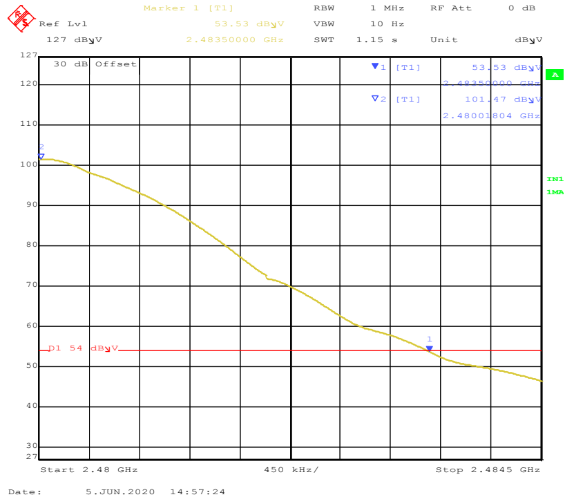
Figure 27: Band-edge-2480 MHz-H-Avg
