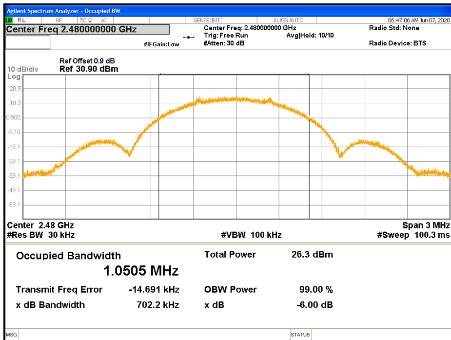
Figure 10: 99% Bandwidth-Transmitter -2480 MHz
