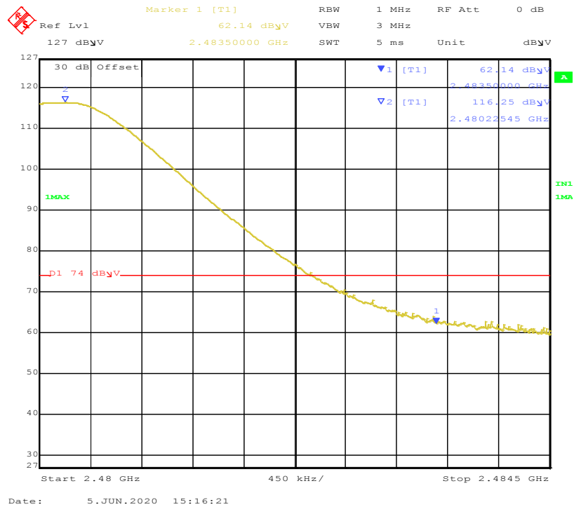
Figure 26: Band-edge-2480 MHz-H-Pk
