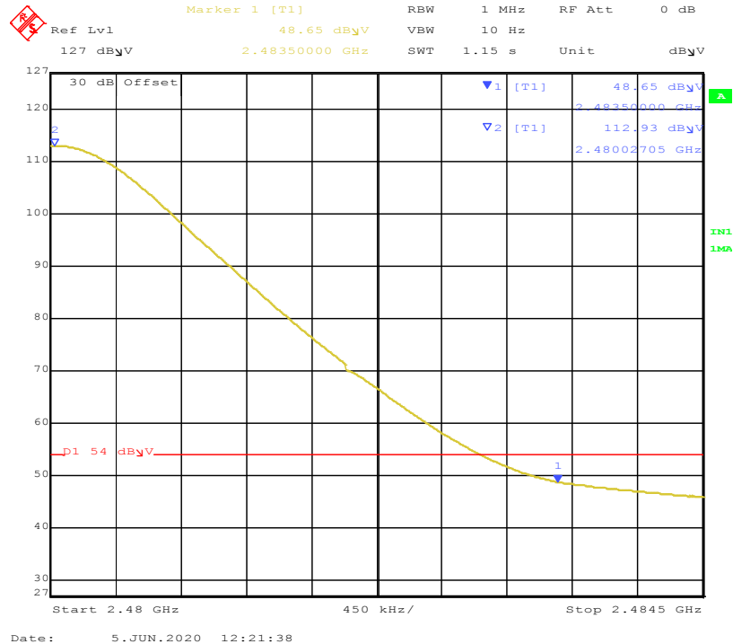
Figure 25: Band-edge-2480 MHz-V-Avg
