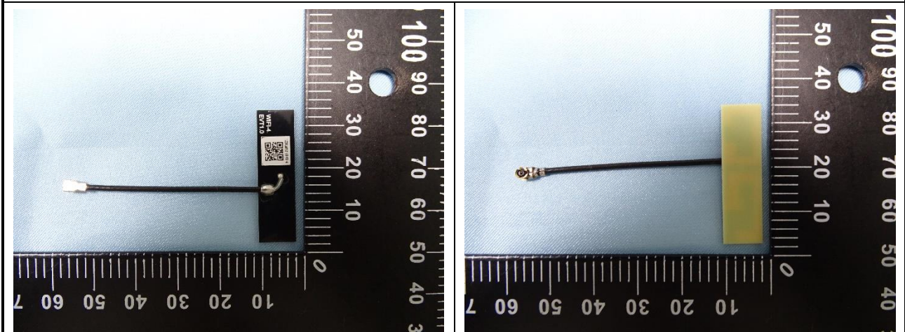
Fig.2 Antenna #2
