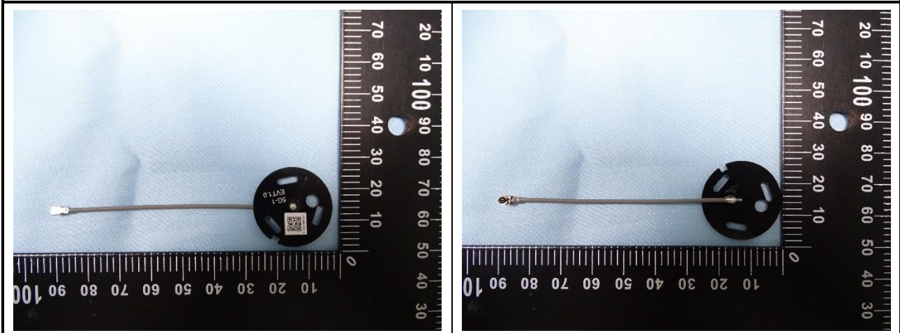
Fig.1 Antenna #1
