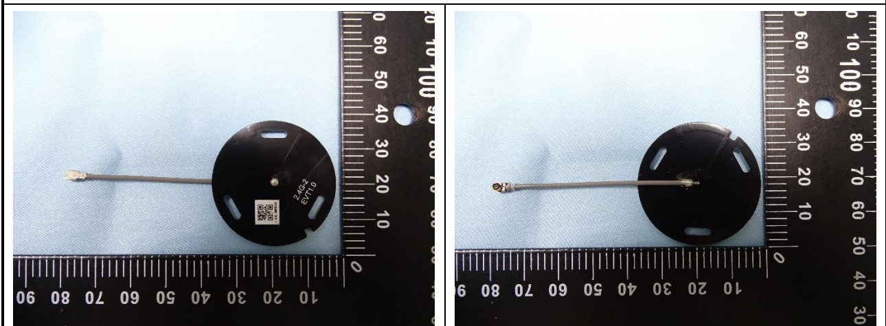
Fig.3 Antenna #3
